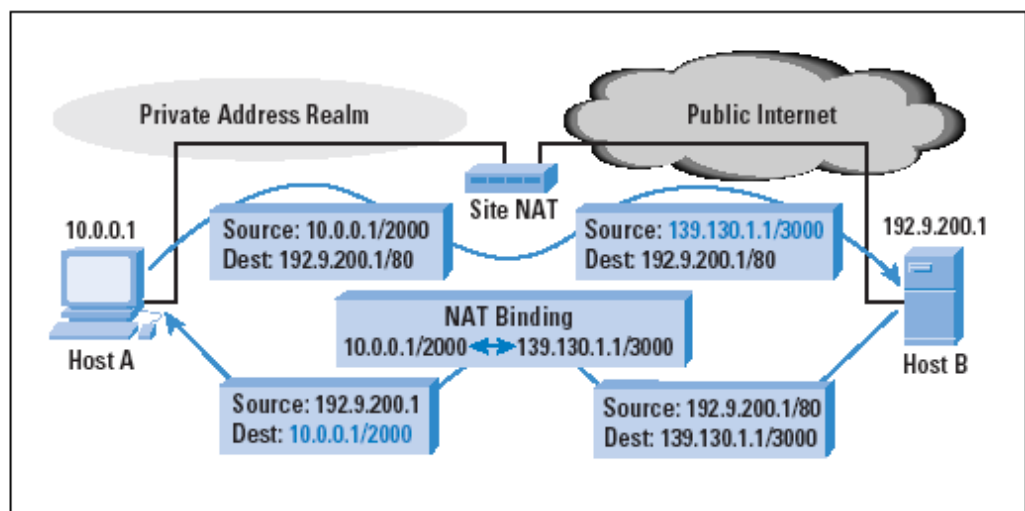
Figure 4: NAPT Traversal
