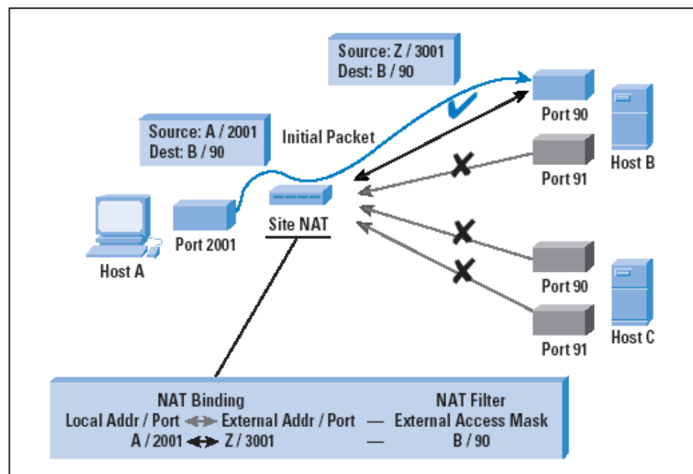
Figure 5: Symmetric NAT
