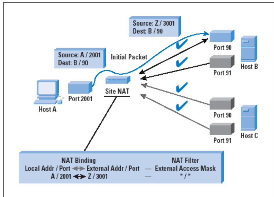
Figure 6: Full Cone NAT
