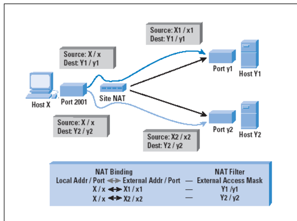
Figure 11: Outbound Connections from a Common Source
