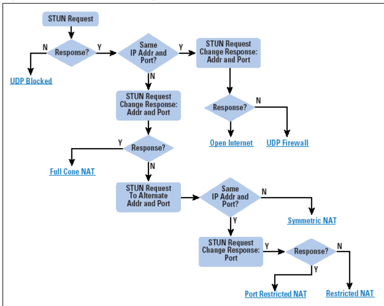
Figure 9: NAT Discovery Process Using STUN
