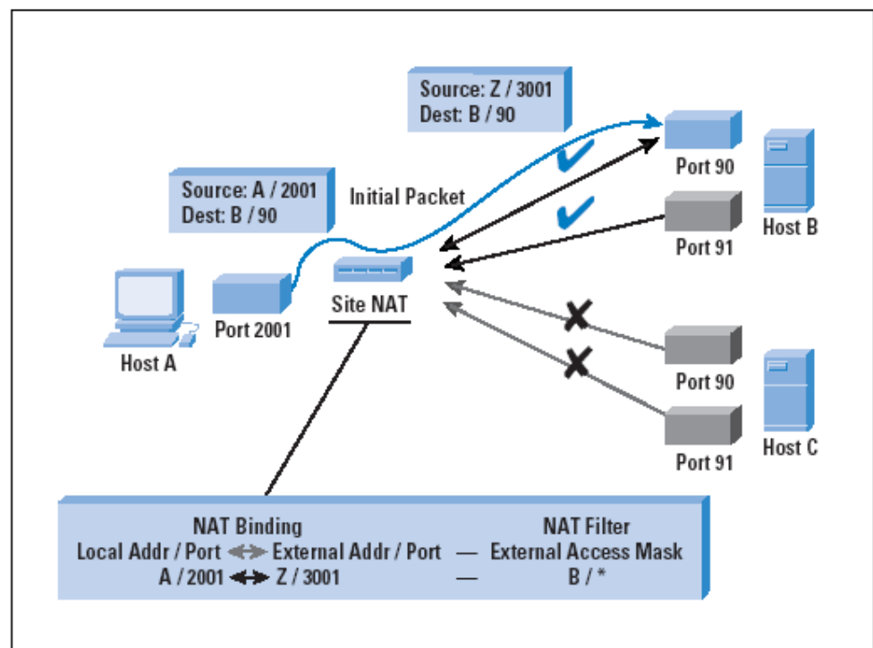
Figure 7: Restricted-Cone NAT
