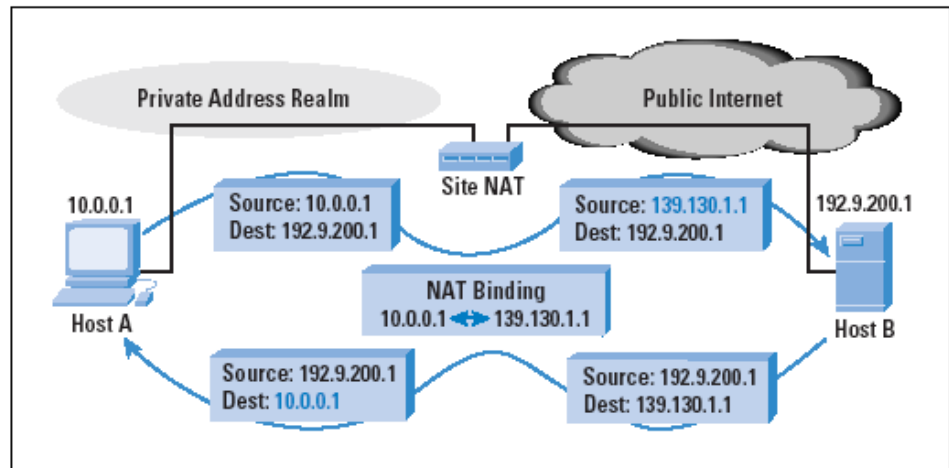
Figure 3: NAT Traversal
