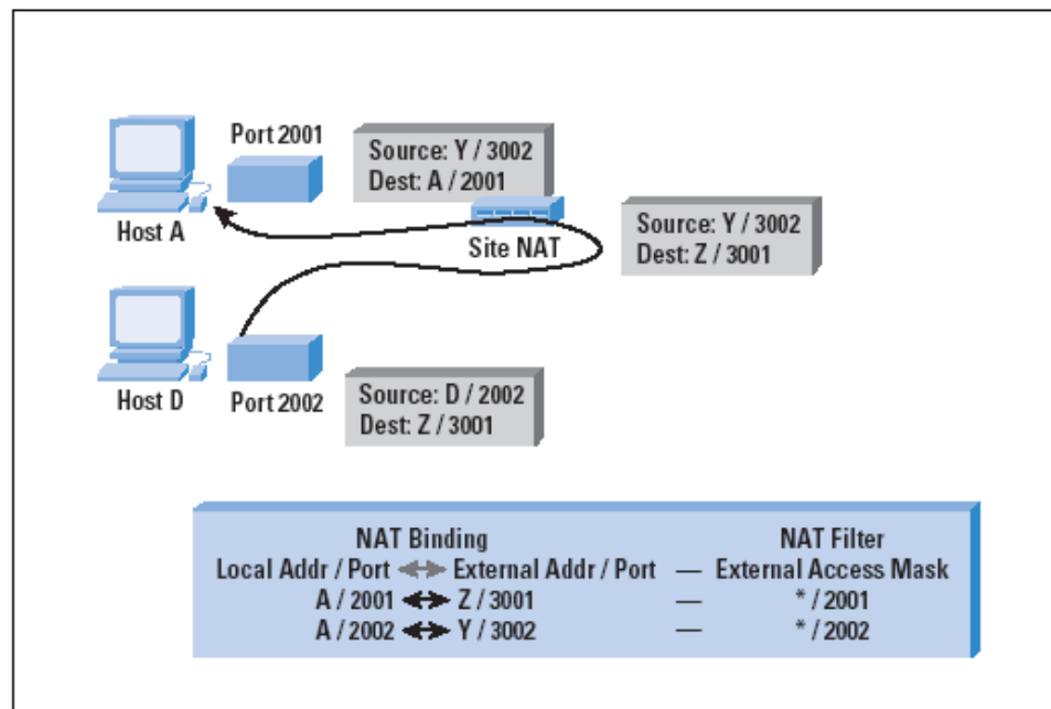
Figure 10: Hairpin NAT Operation
