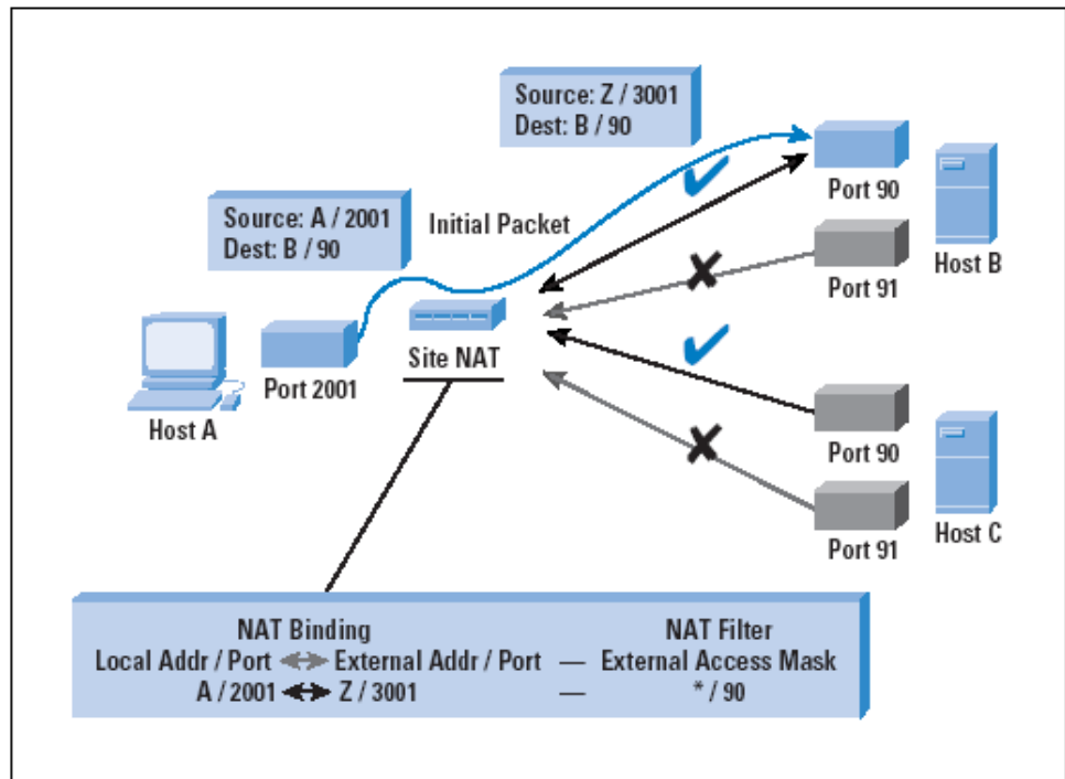
Figure 8: Port-Restricted-Cone NAT
