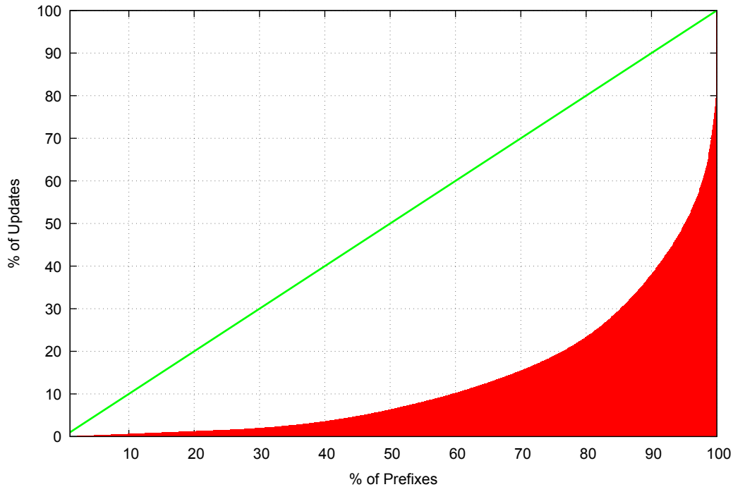
BGP v4 Prefix Update Cumulative Distribution
