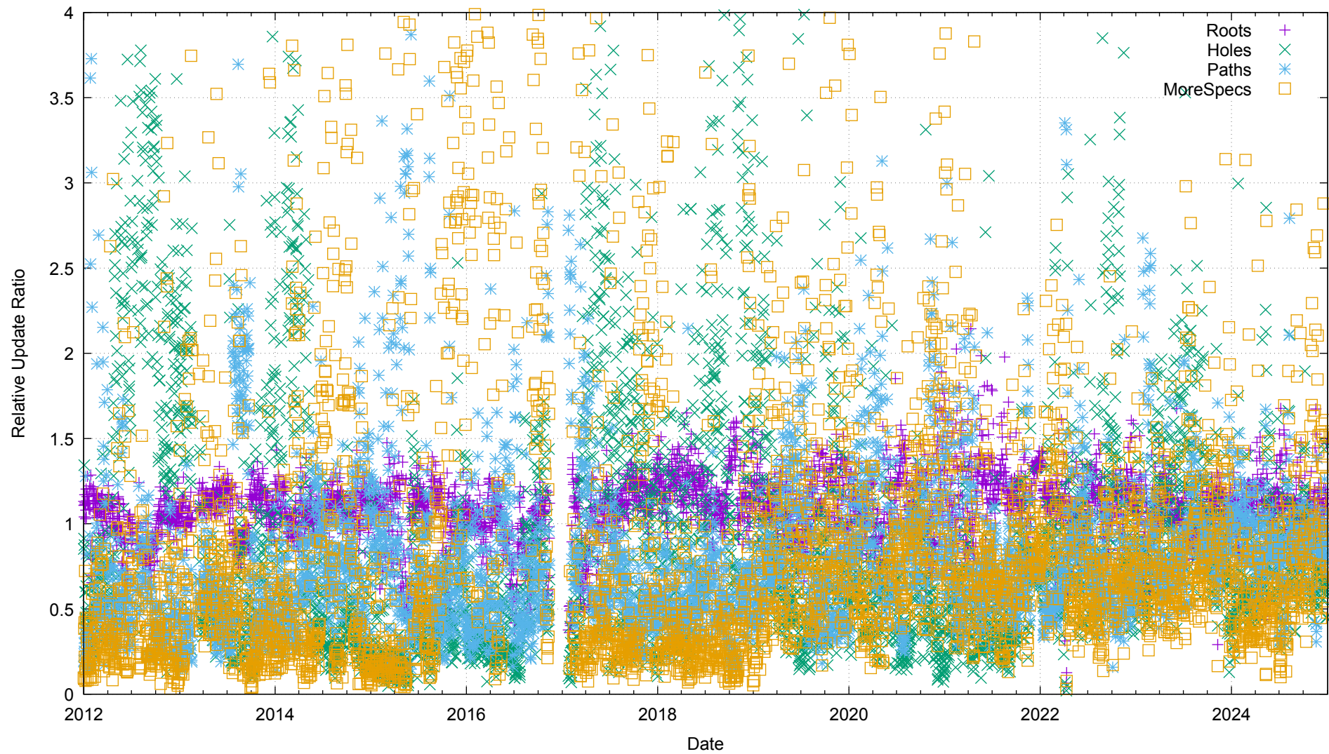
BGP v6 Prefix Profile
