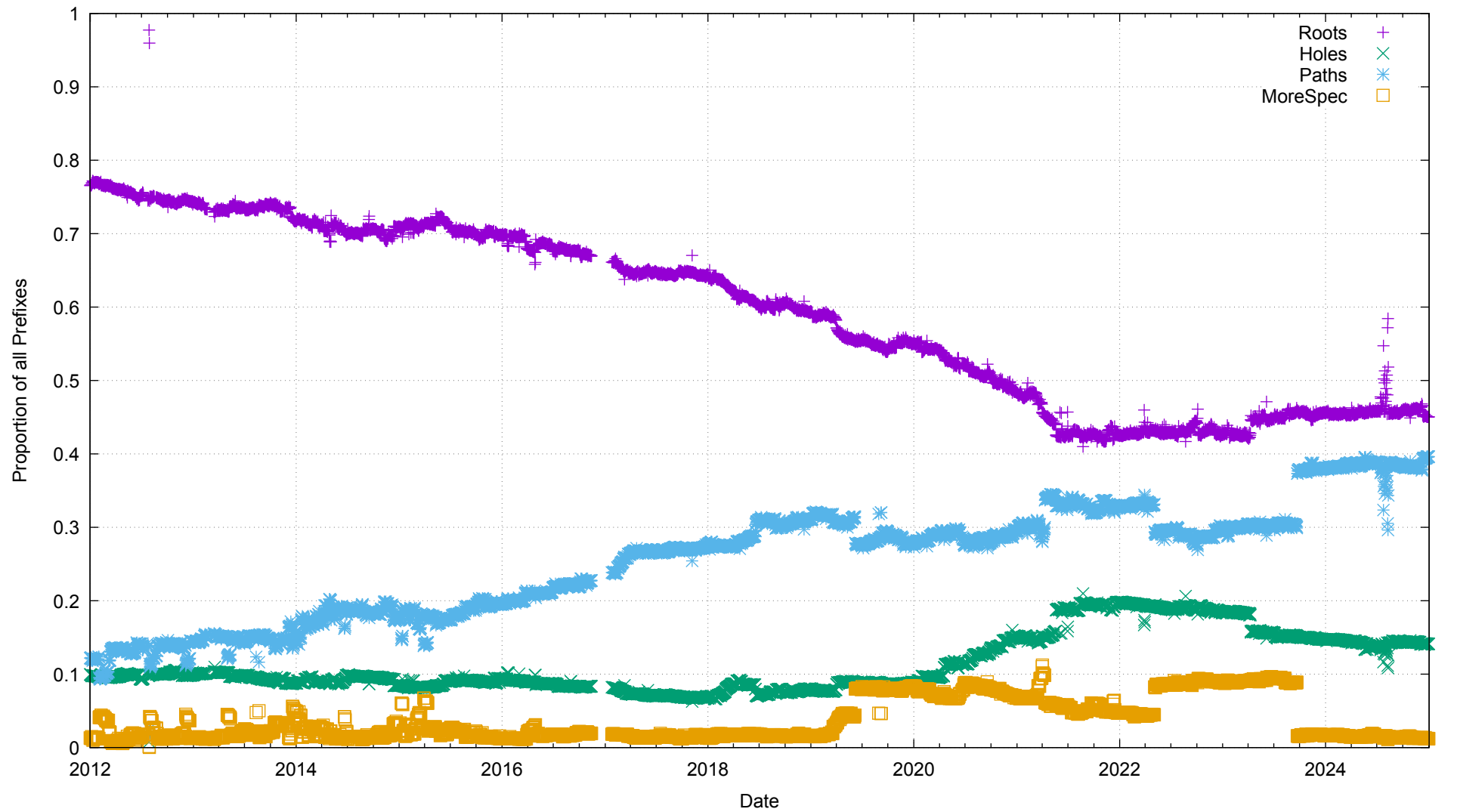
BGP v6 Prefix Profile
