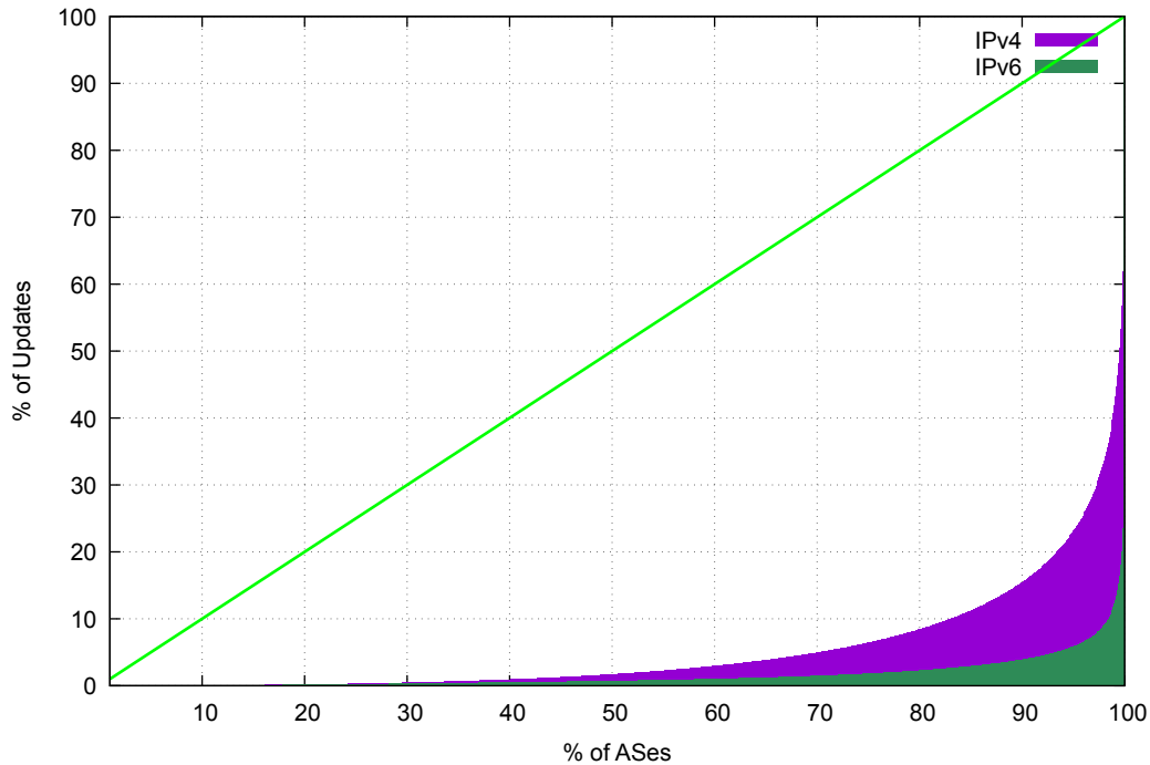
BGP v6 AS Update Cumulative Distribution
