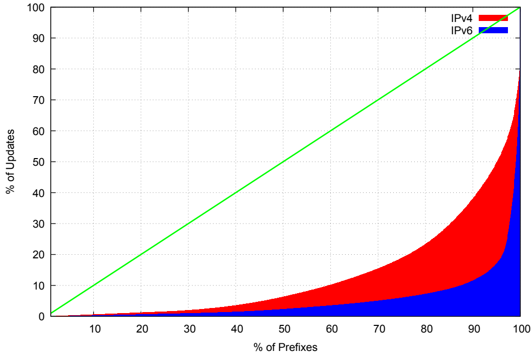
BGP v6 Prefix Update Cumulative Distribution
