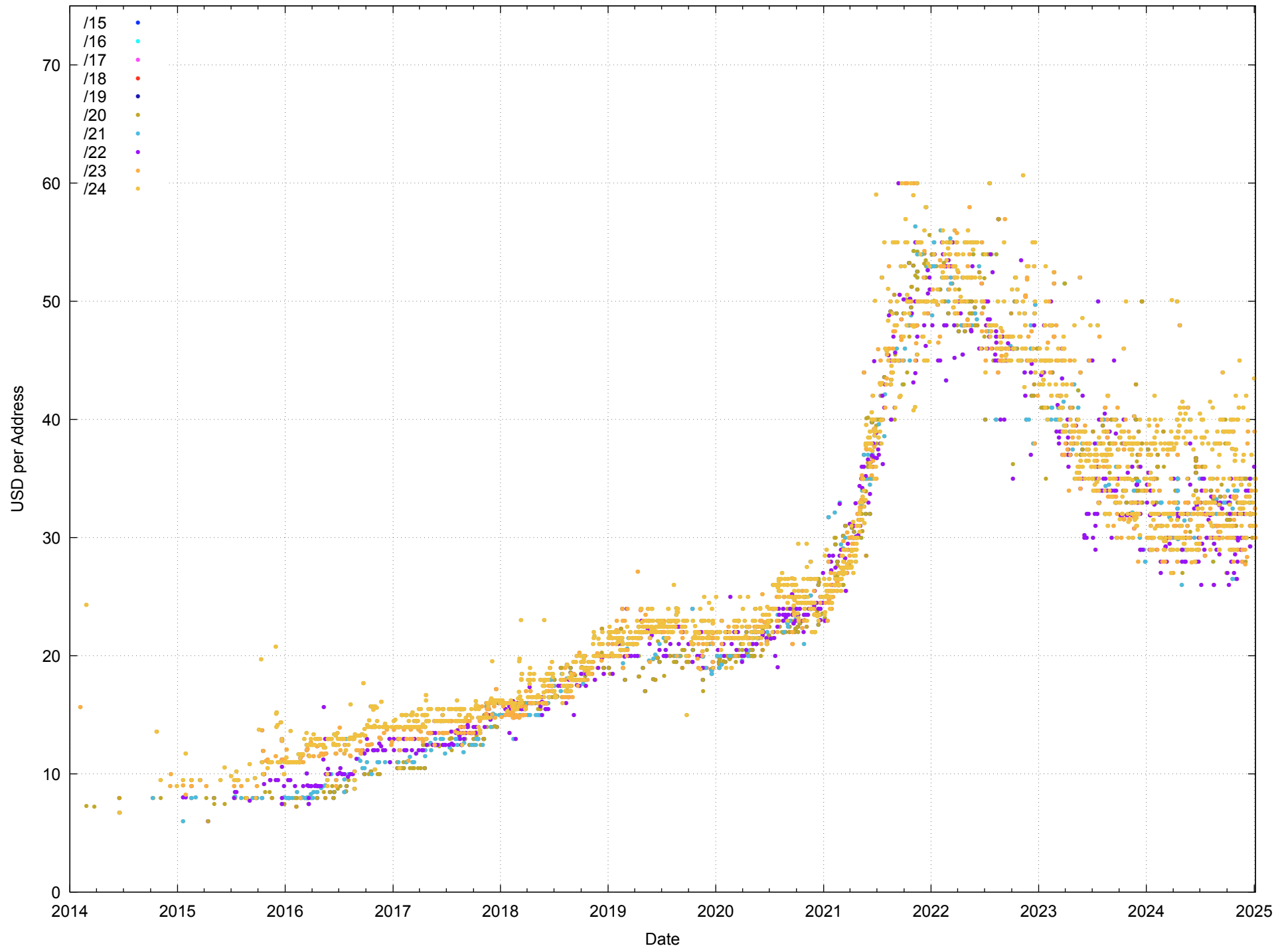
Unit Price of Traded IPv4 Addresses (From Hilco Streambank)
