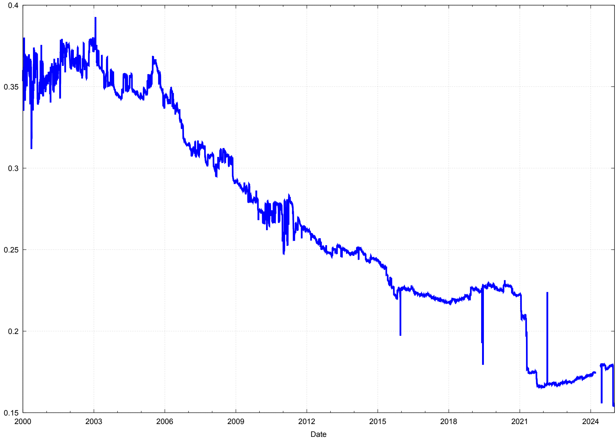
IPv4 Unadvertised Address Ratio
