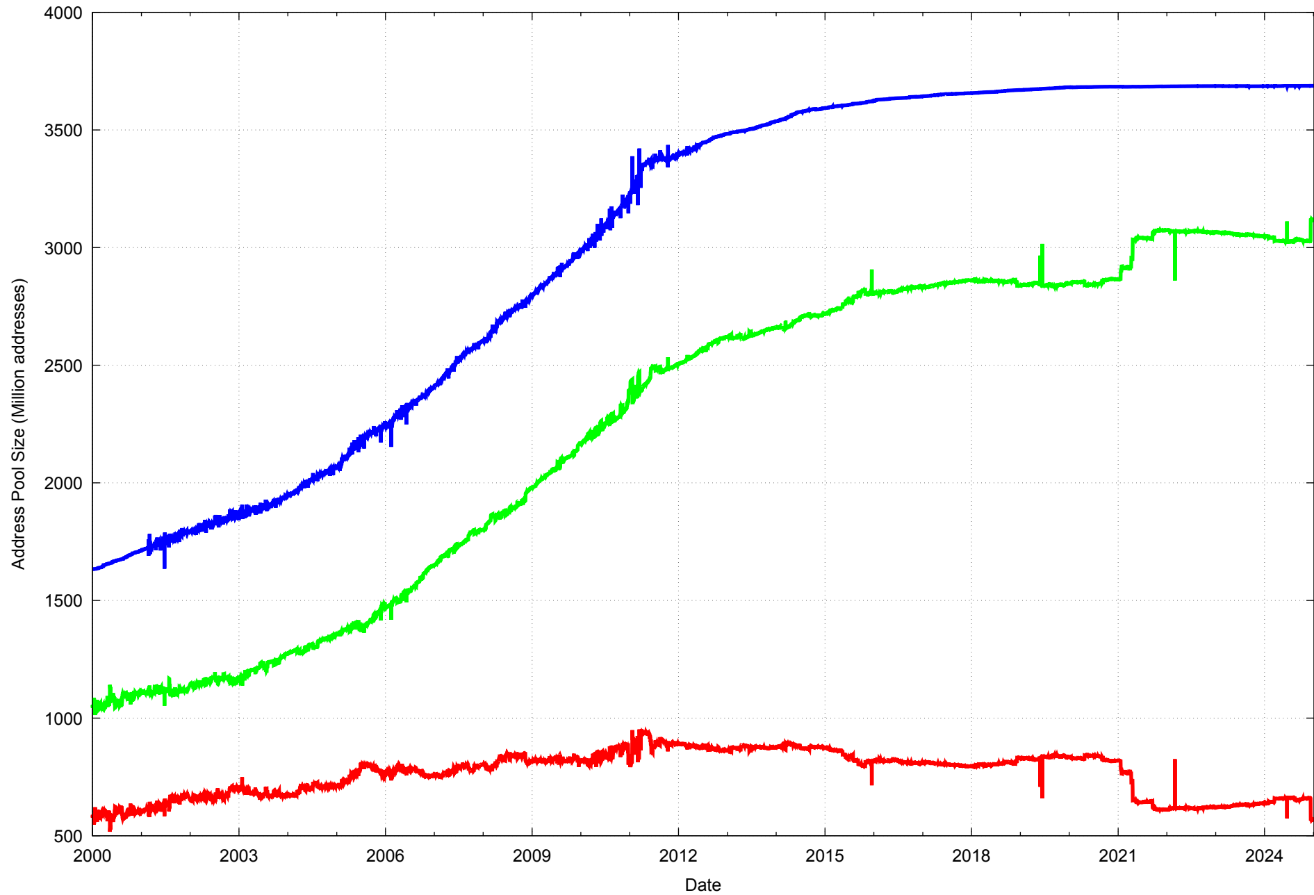
Unadvertised IPv4 Addresses
