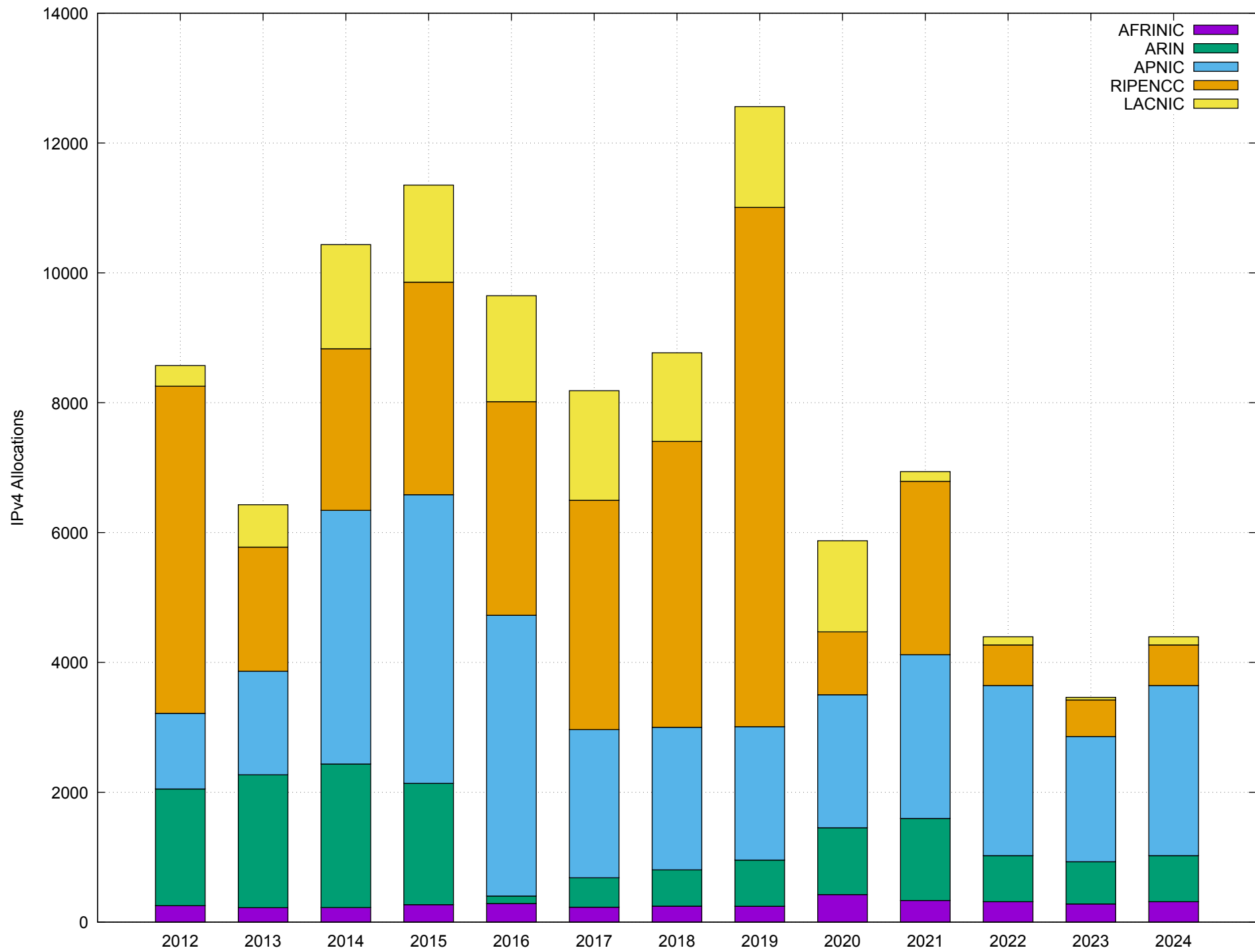
IPv4 Address Allocations by RIR 2012 - 2024
