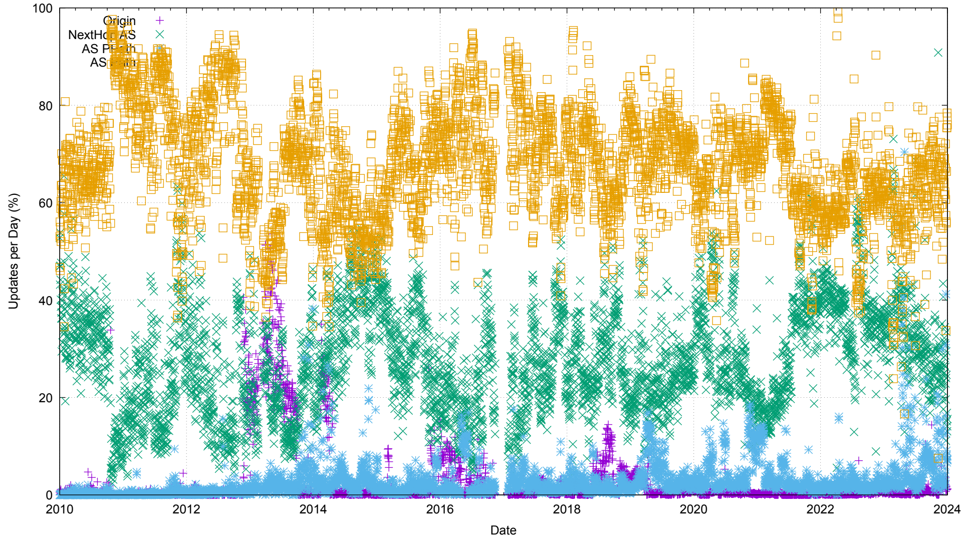
BGP v6 Daily Update Profile
