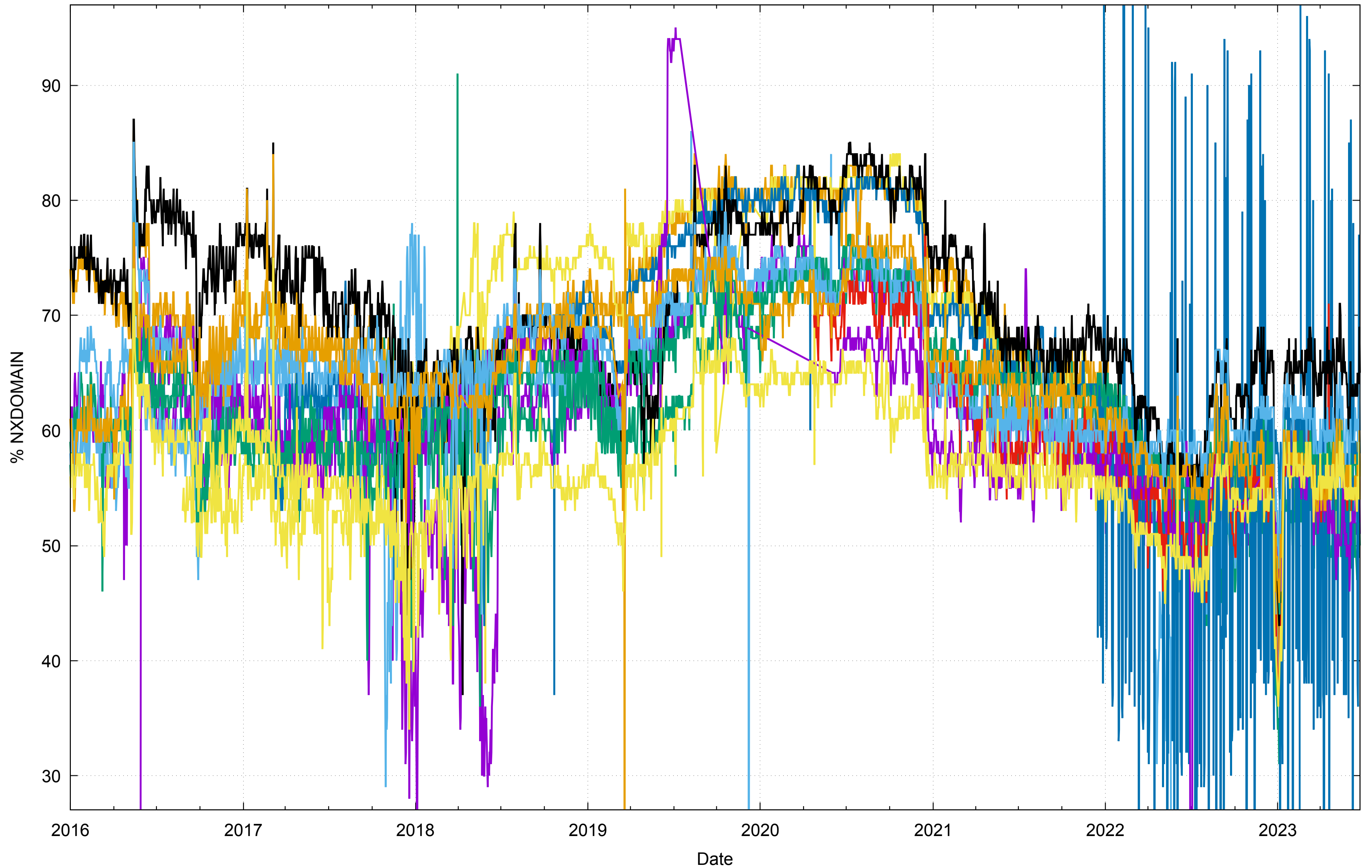
NXDOMAIN response rate - Root Servers
