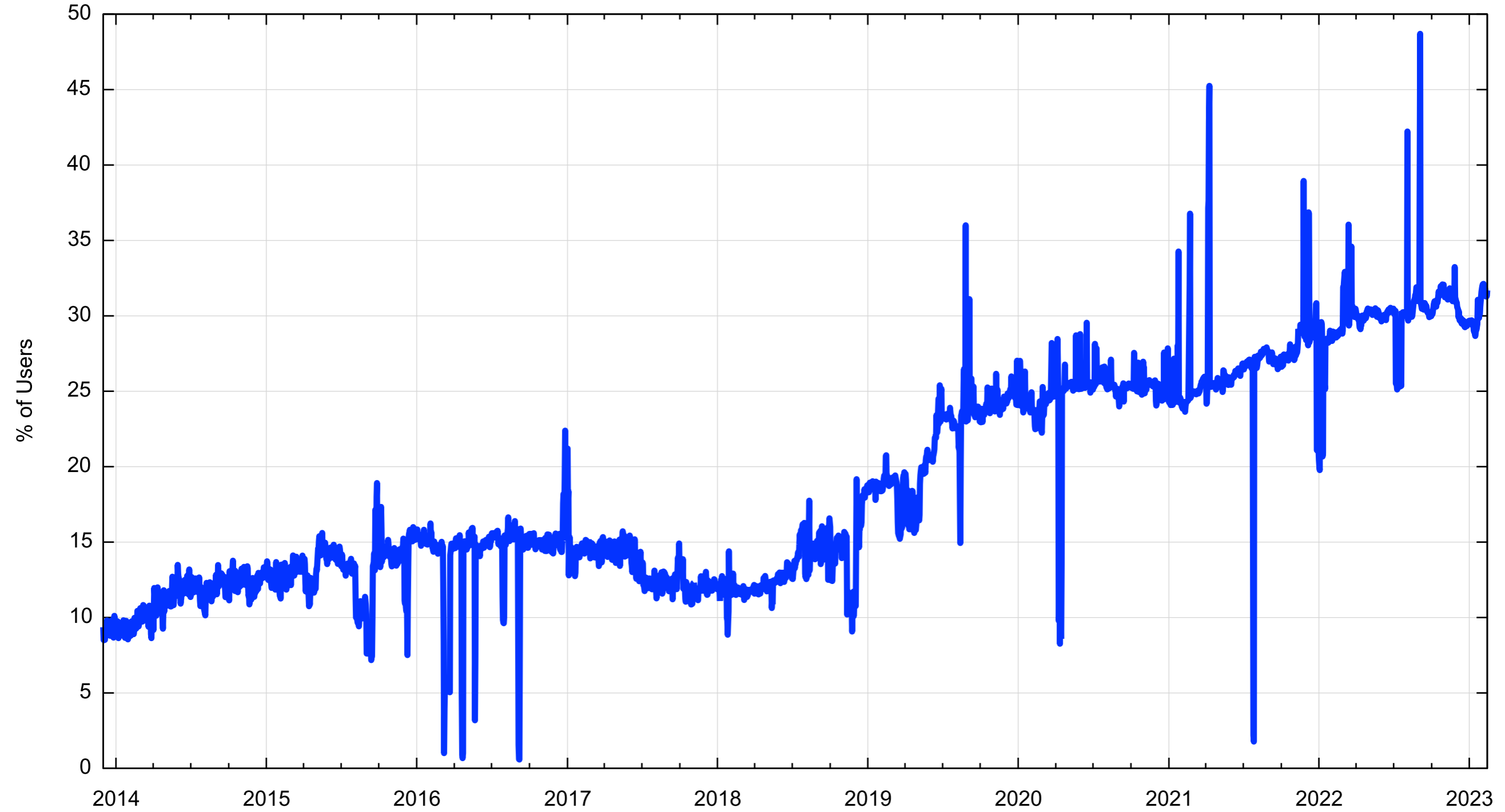
DNSSEC Validation Rates - 2013 - 2023
