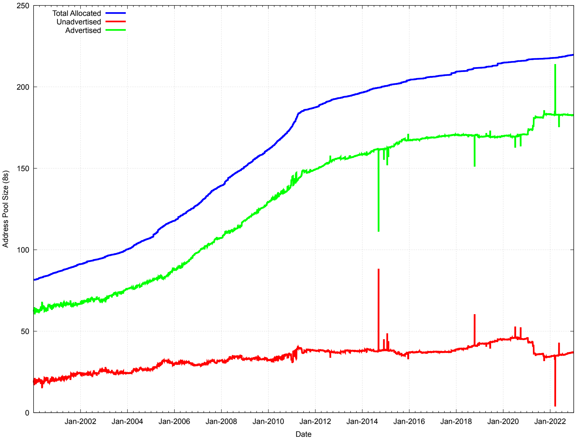
IPv4 Address Pool Sizes - 2000 - 2022
