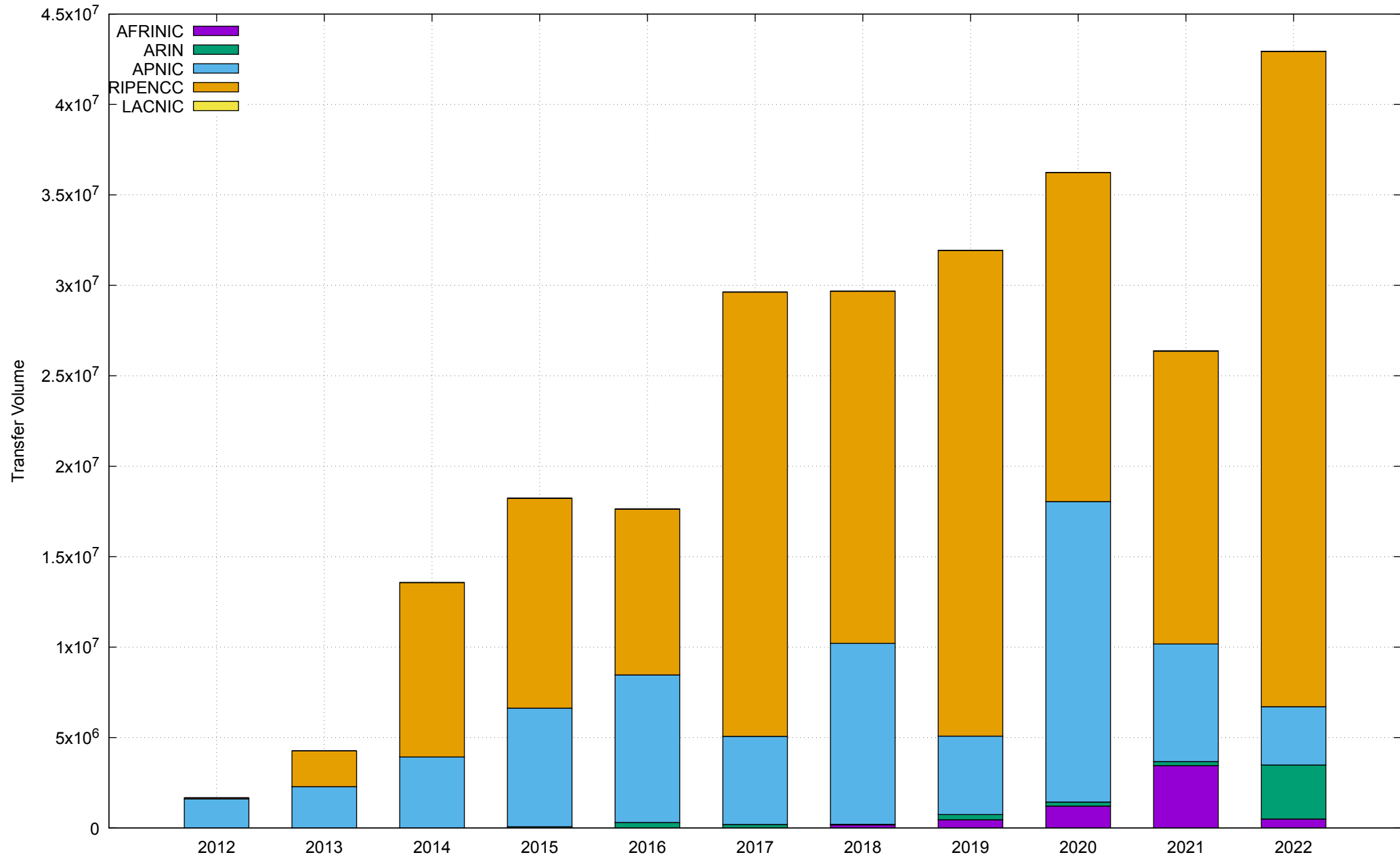
IPv4 Transfers, 2012 - 2022
