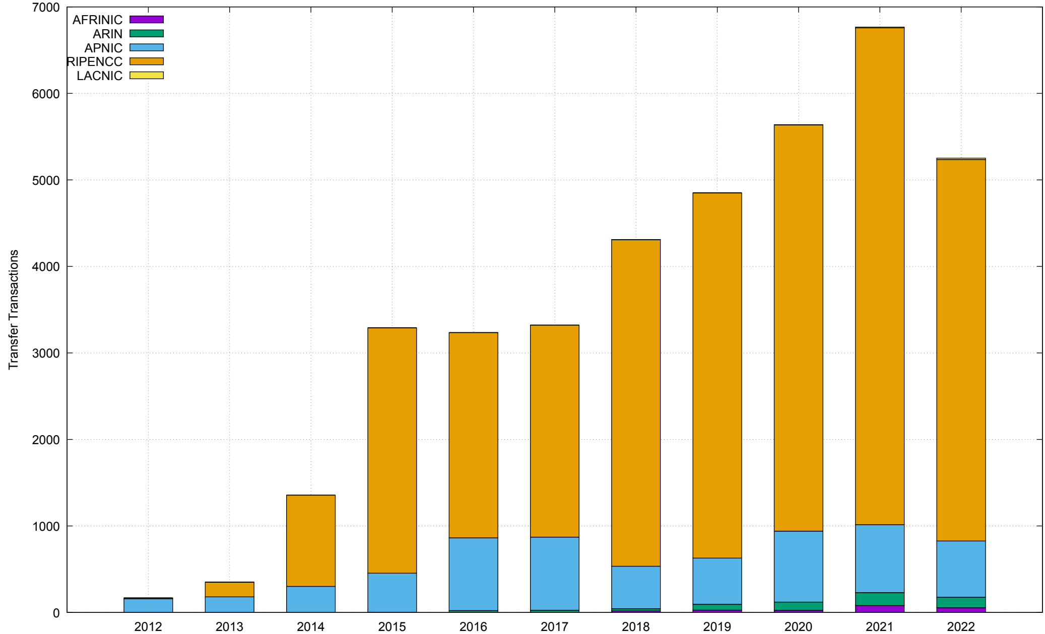
IPv4 Transfers, 2012 - 2022
