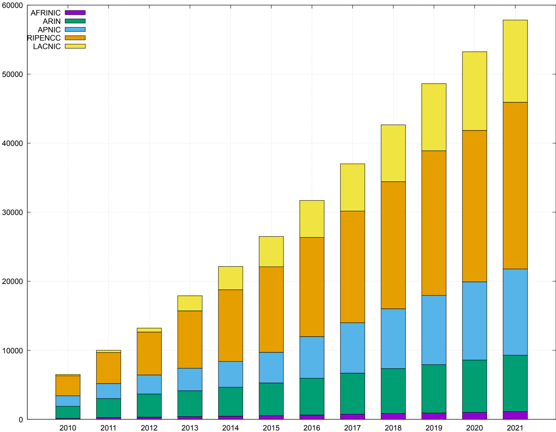
IPv6 Allocations by RIR 2010 - 2021
