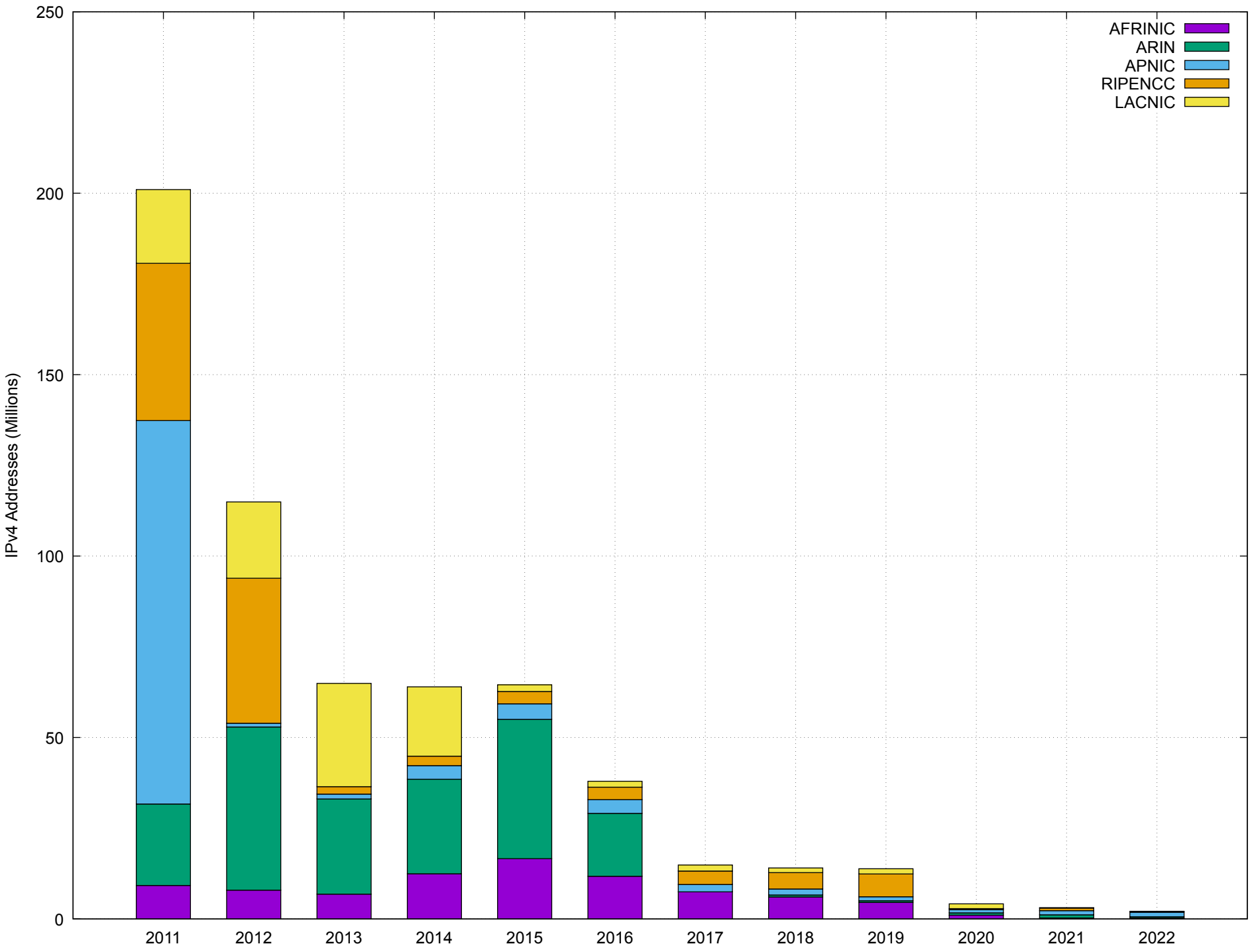
IPv4 Address Allocations by RIR 2011 - 2022
