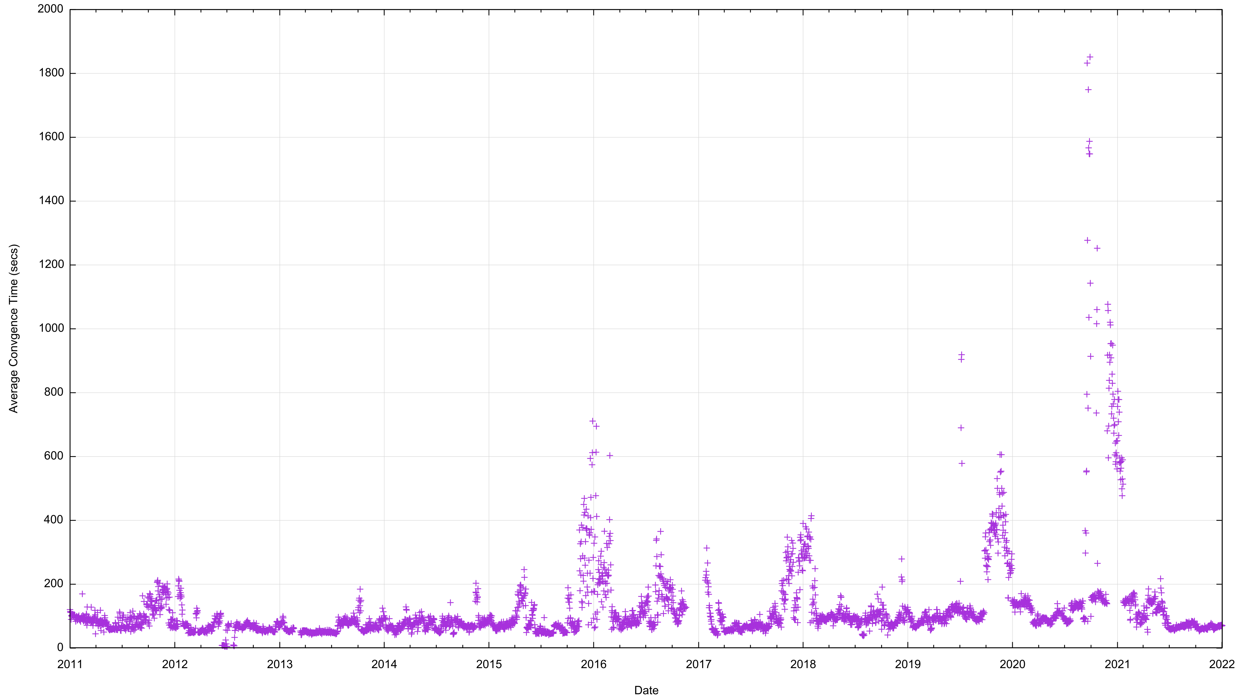
Daily Average BGP IPv6 Convergence Time
