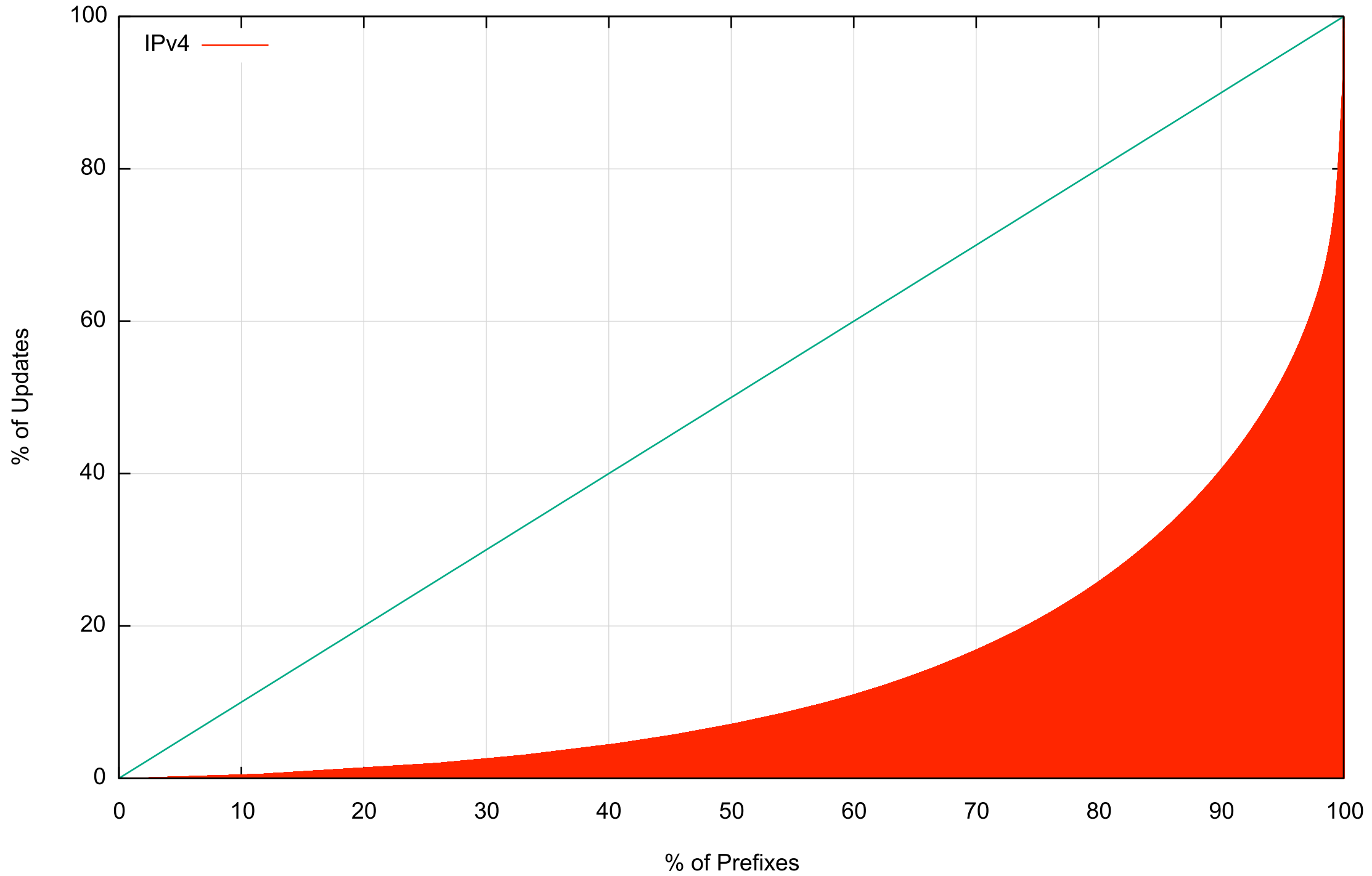
BGP IPv4 Update Distribution by Prefix
