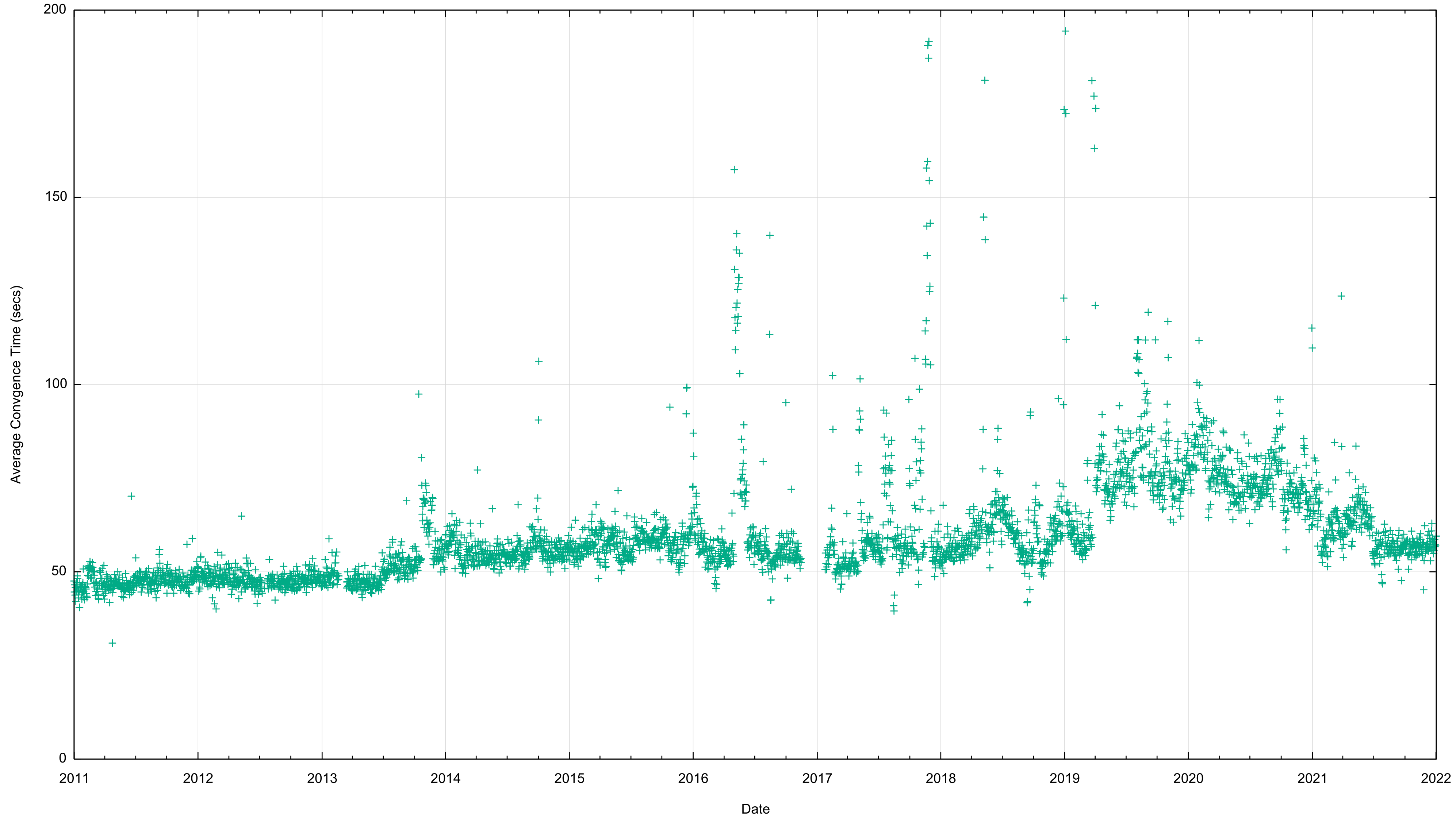
Daily Average BGP IPv4 Convergence Time
