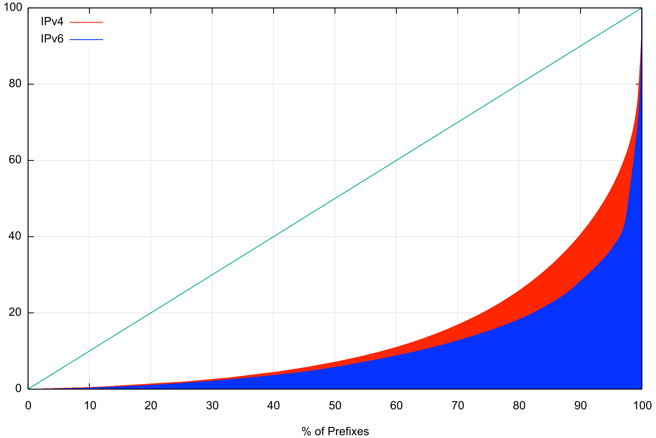
BGP IPv4 and IPv6 Update Distribution by Prefix
