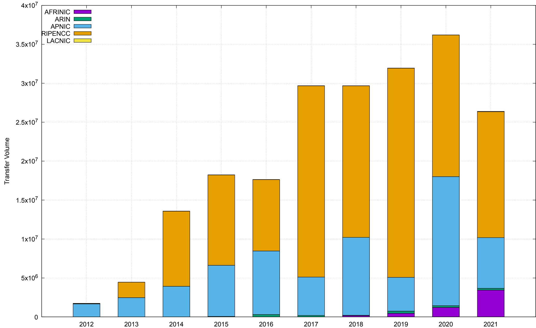
IPv4 Transfers, 2012 - 2021
