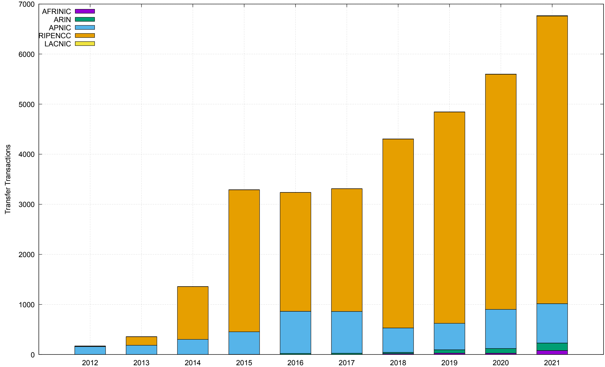
IPv4 Transfers, 2012 - 2021
