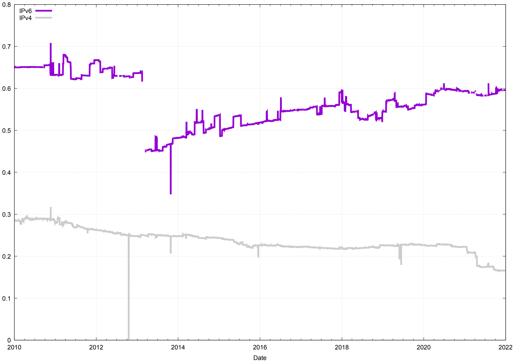
IPv6 UnAdvertised Address Ratio
