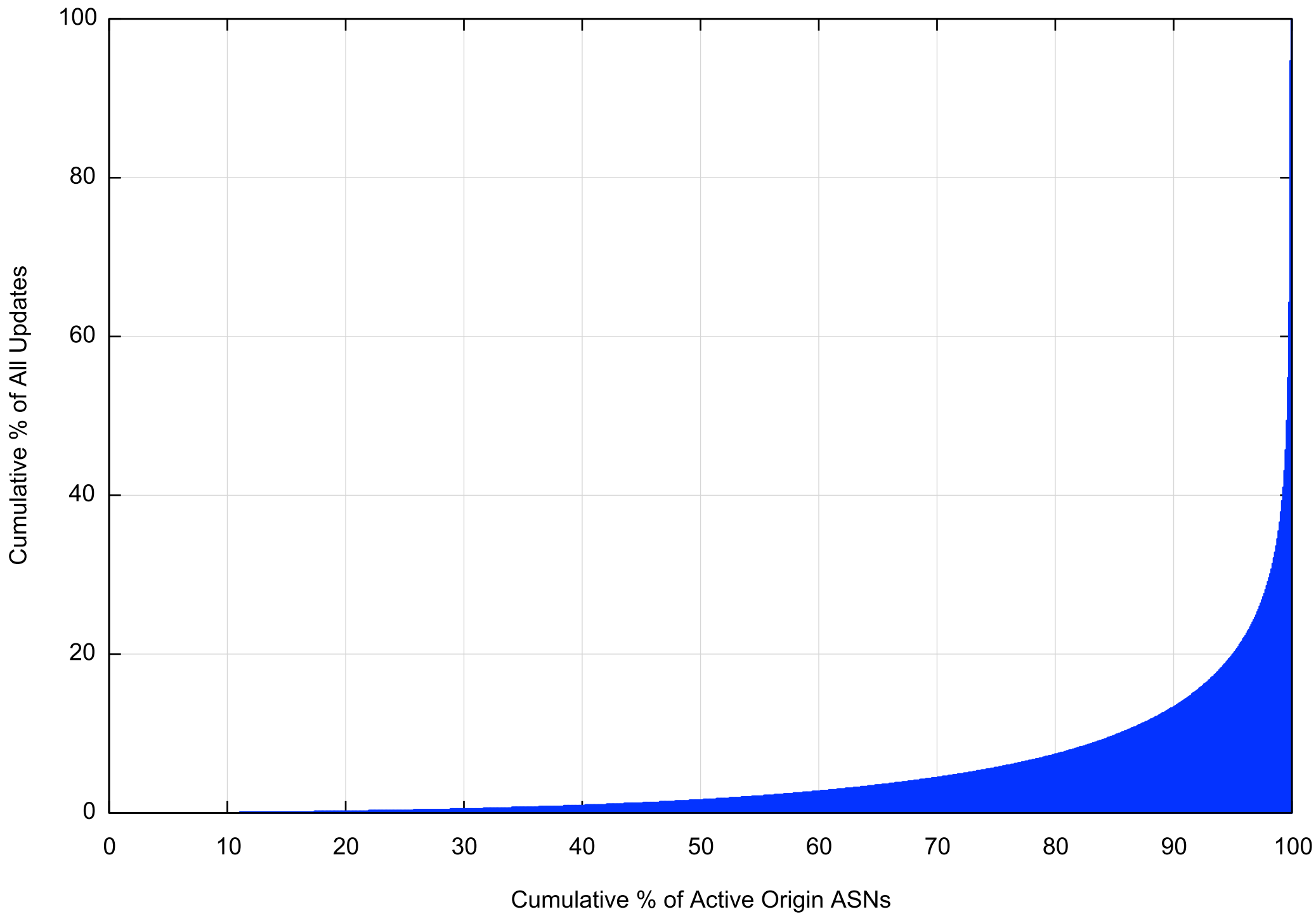
Distribution of Active Origin ASNs to Updates
