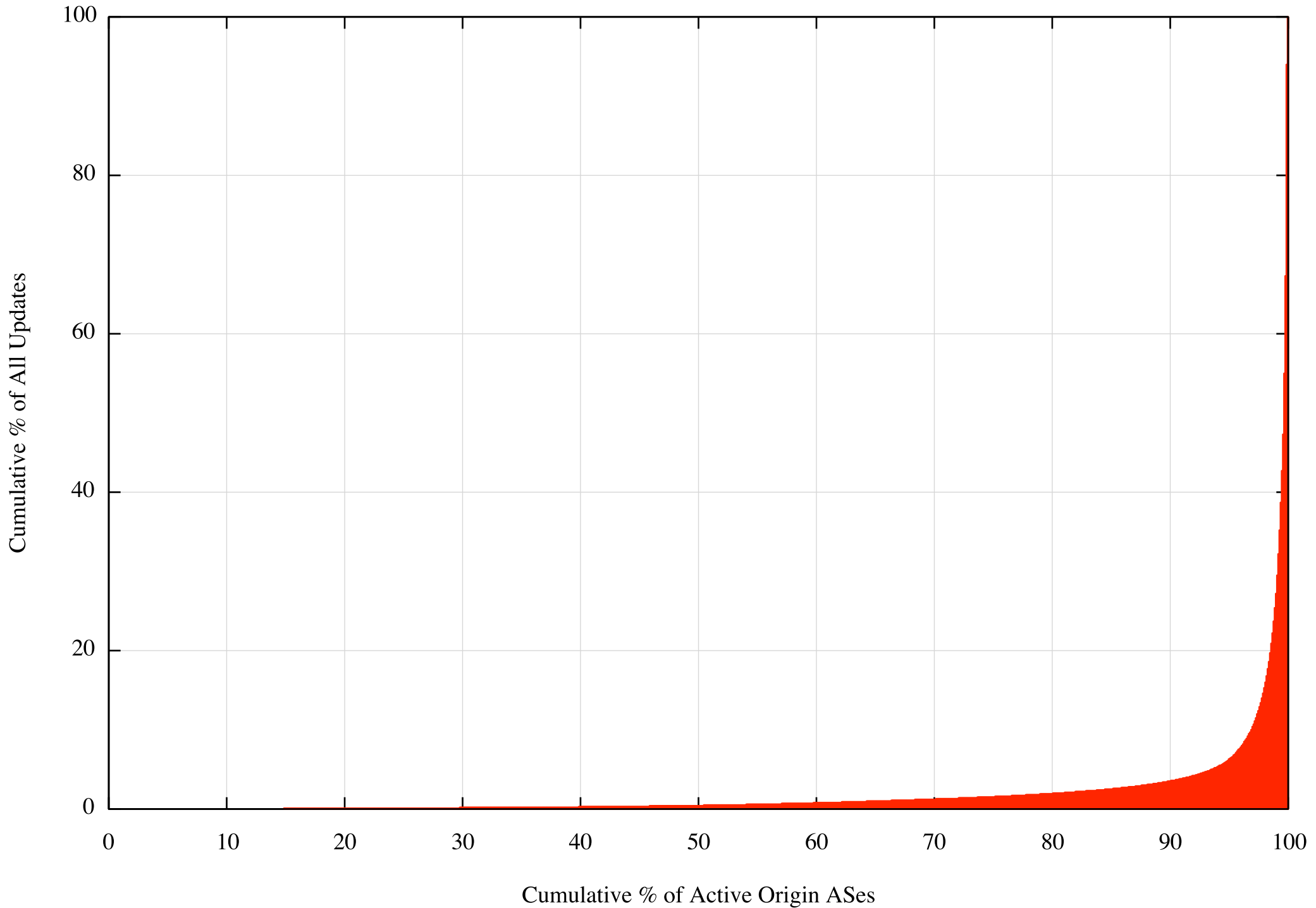
Distribution of Active Origin ASes to Updates
