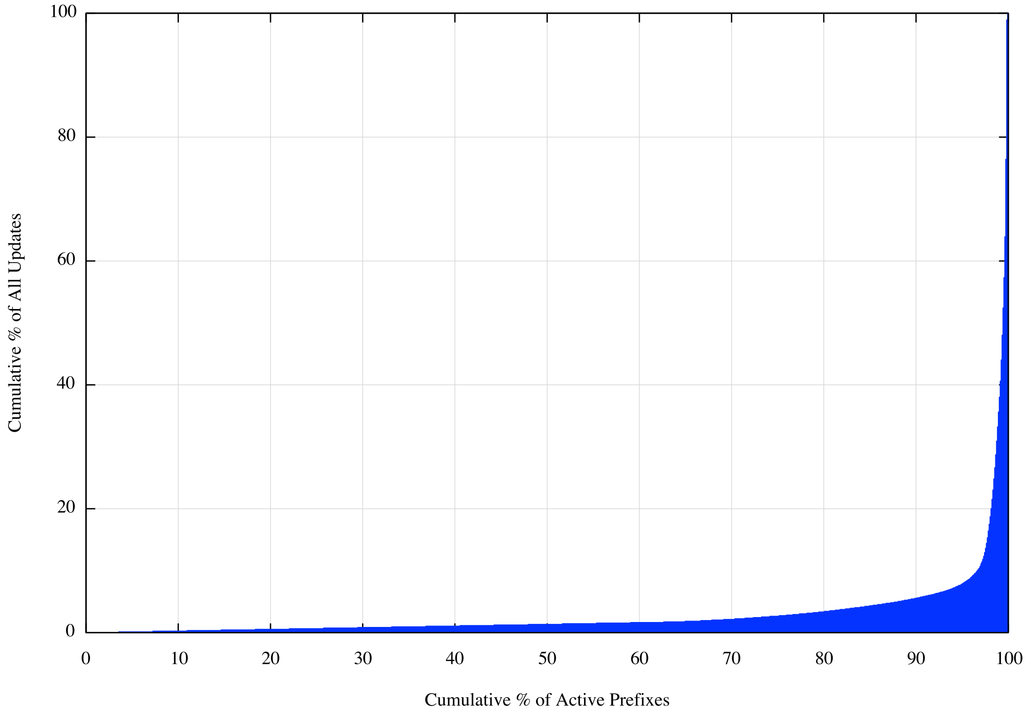
Distribution of Active Prefixes to Updates
