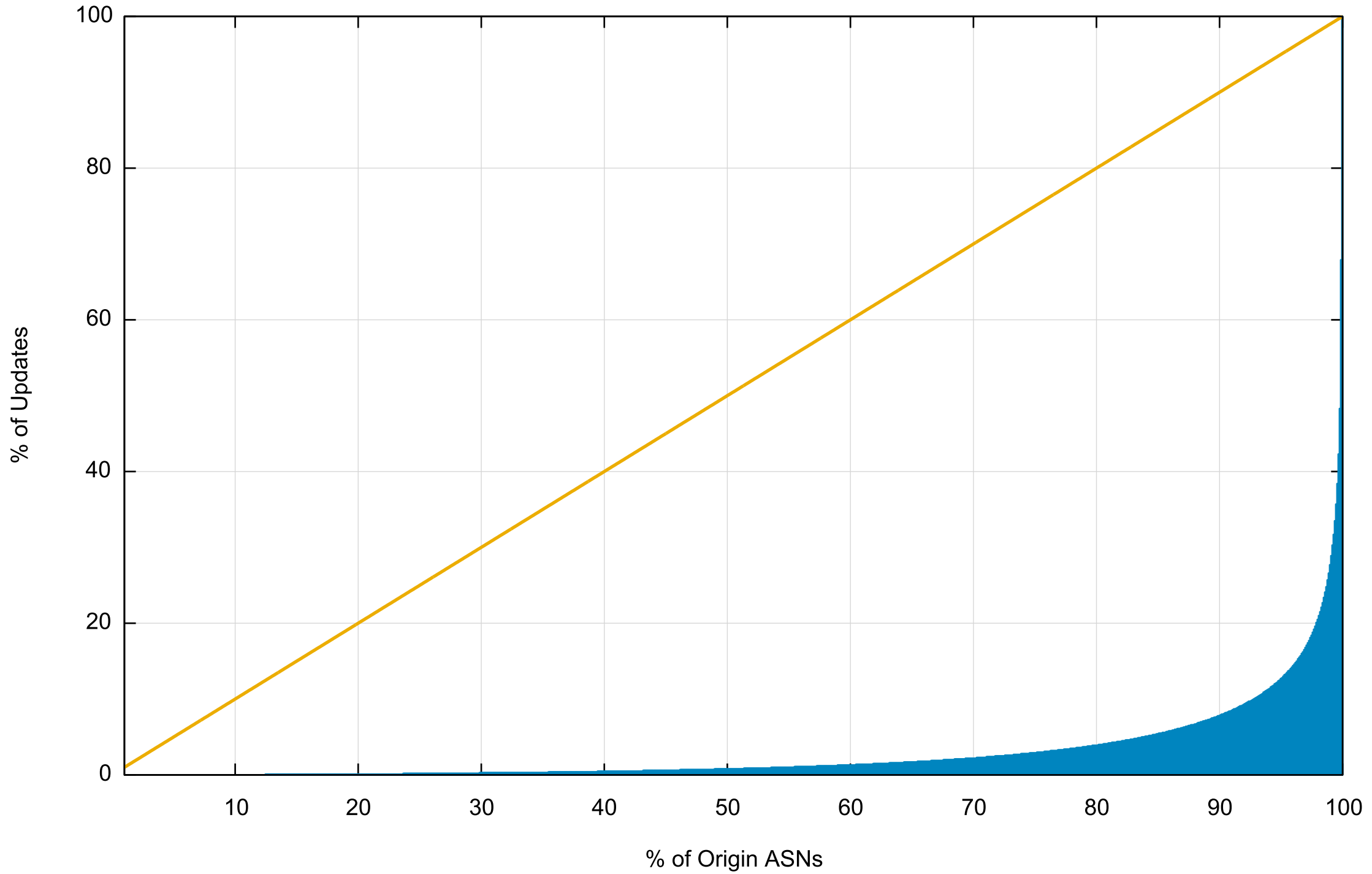
BGP Origin ASN Update Cumulative Distribution
