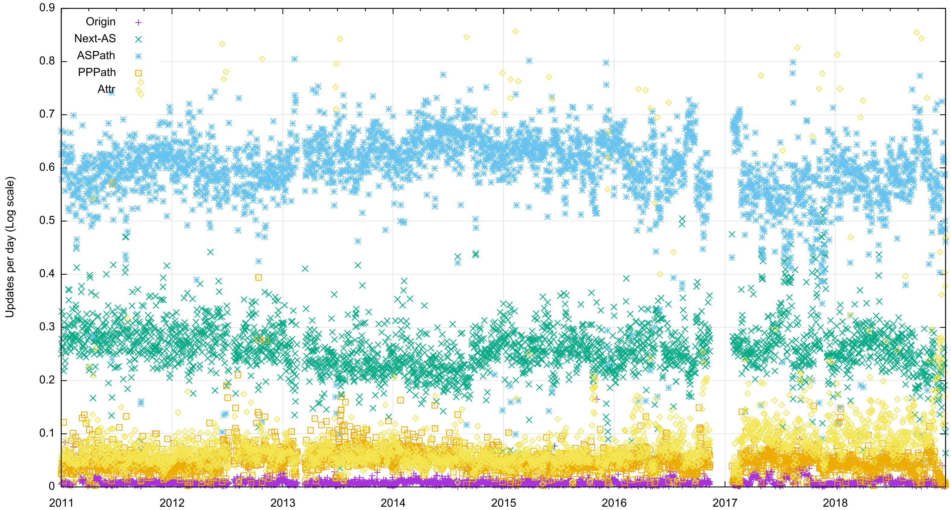
IPv4 Update Profile - Relative Count
