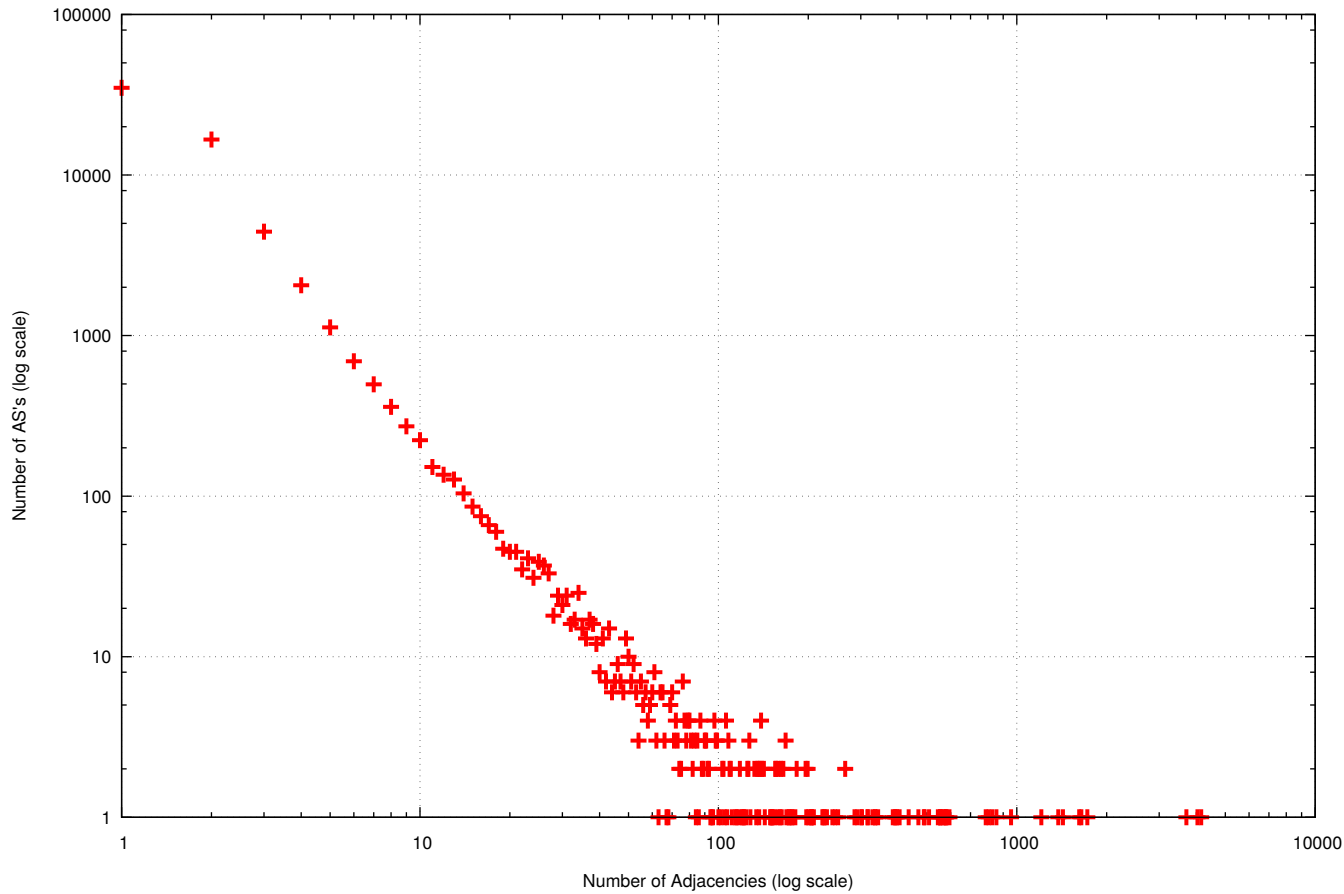
BGP AS Adjacency Distribution
