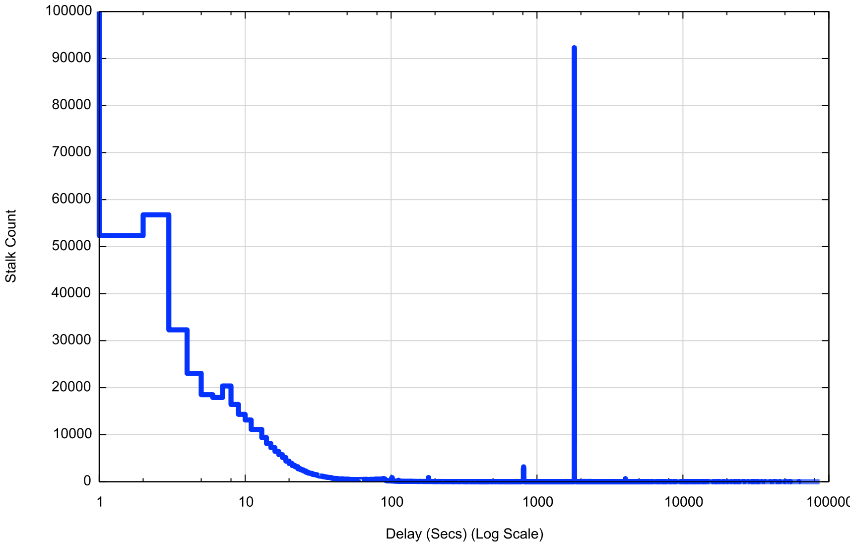
Distribution of Stalking Delay
