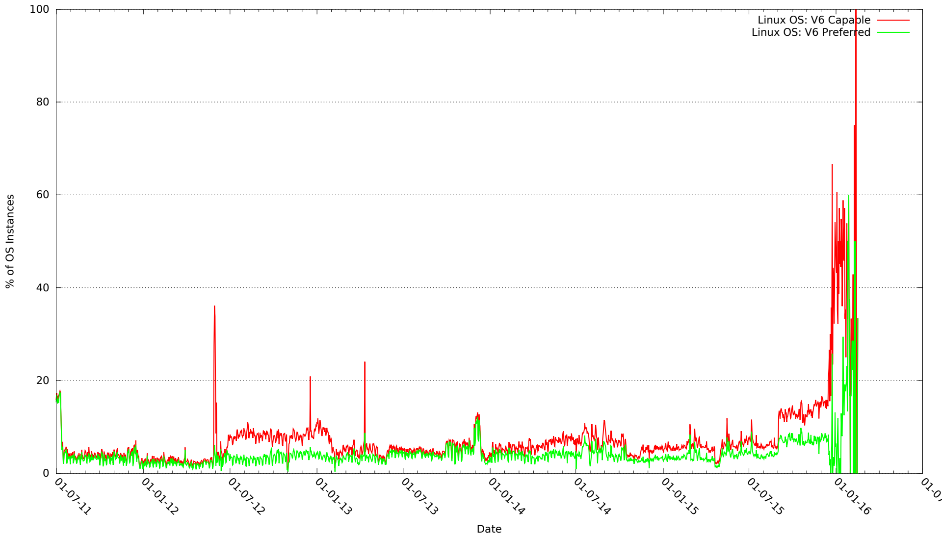
V6 Linux OS Capability
