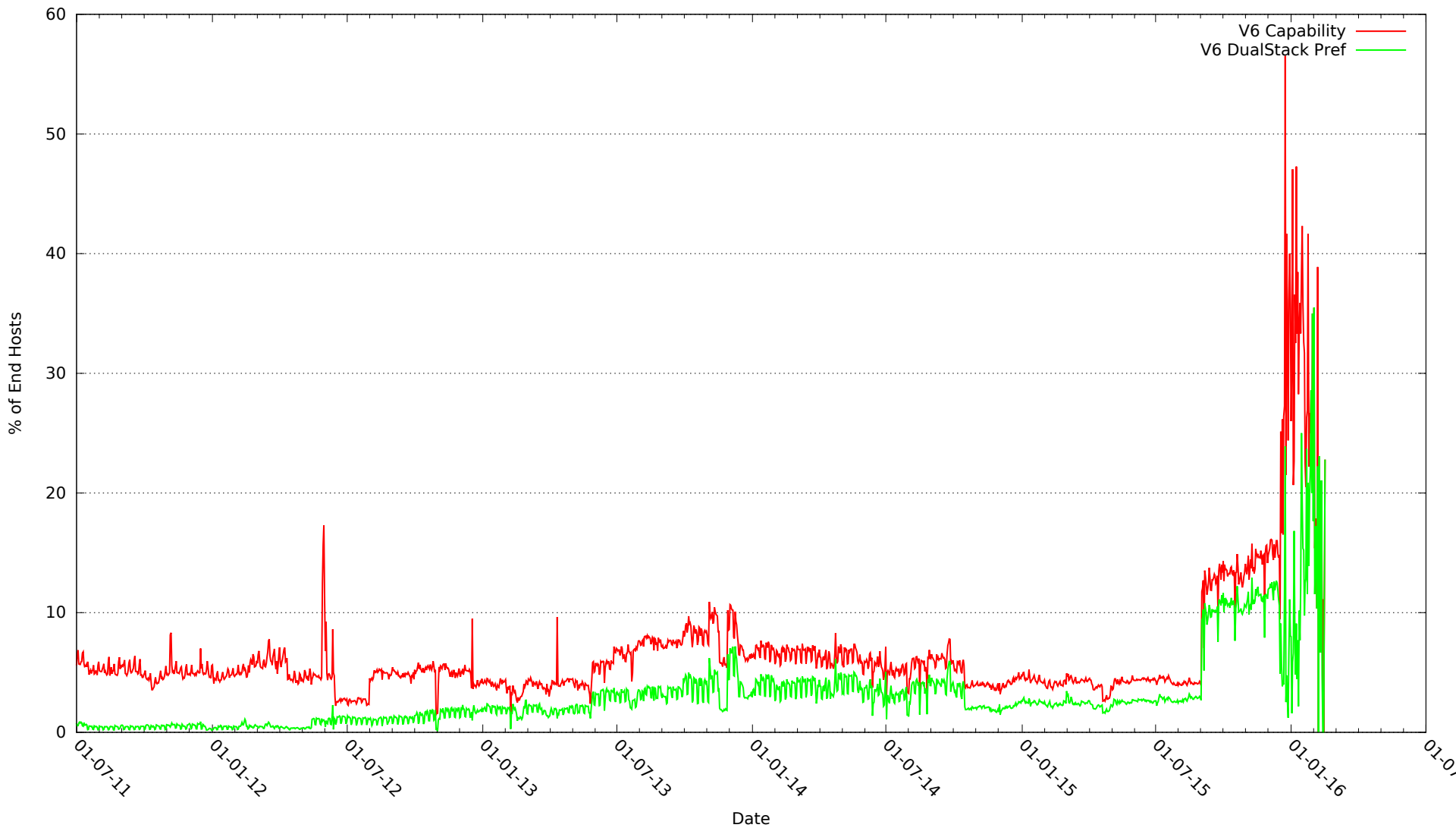
IPv6-Capable End Hosts
