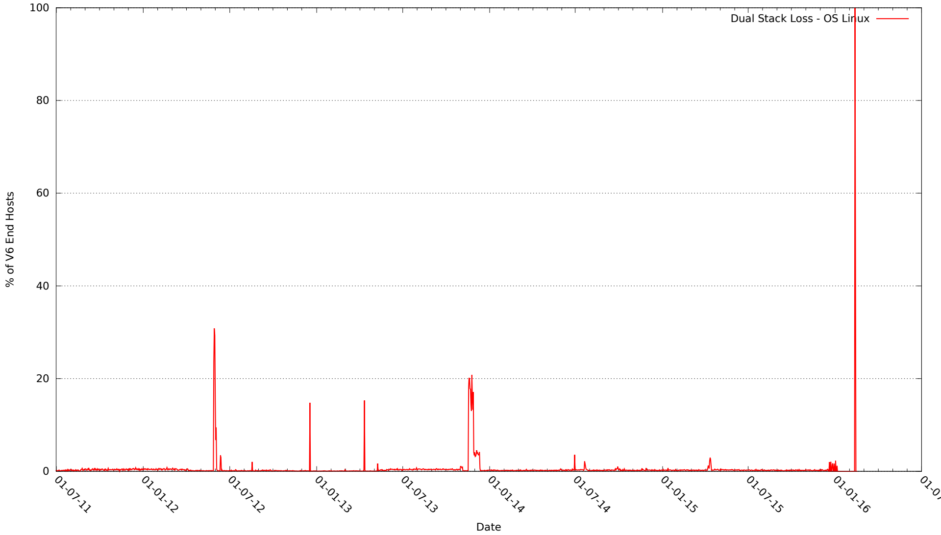
Dual Stack Loss Rate - OS Linux
