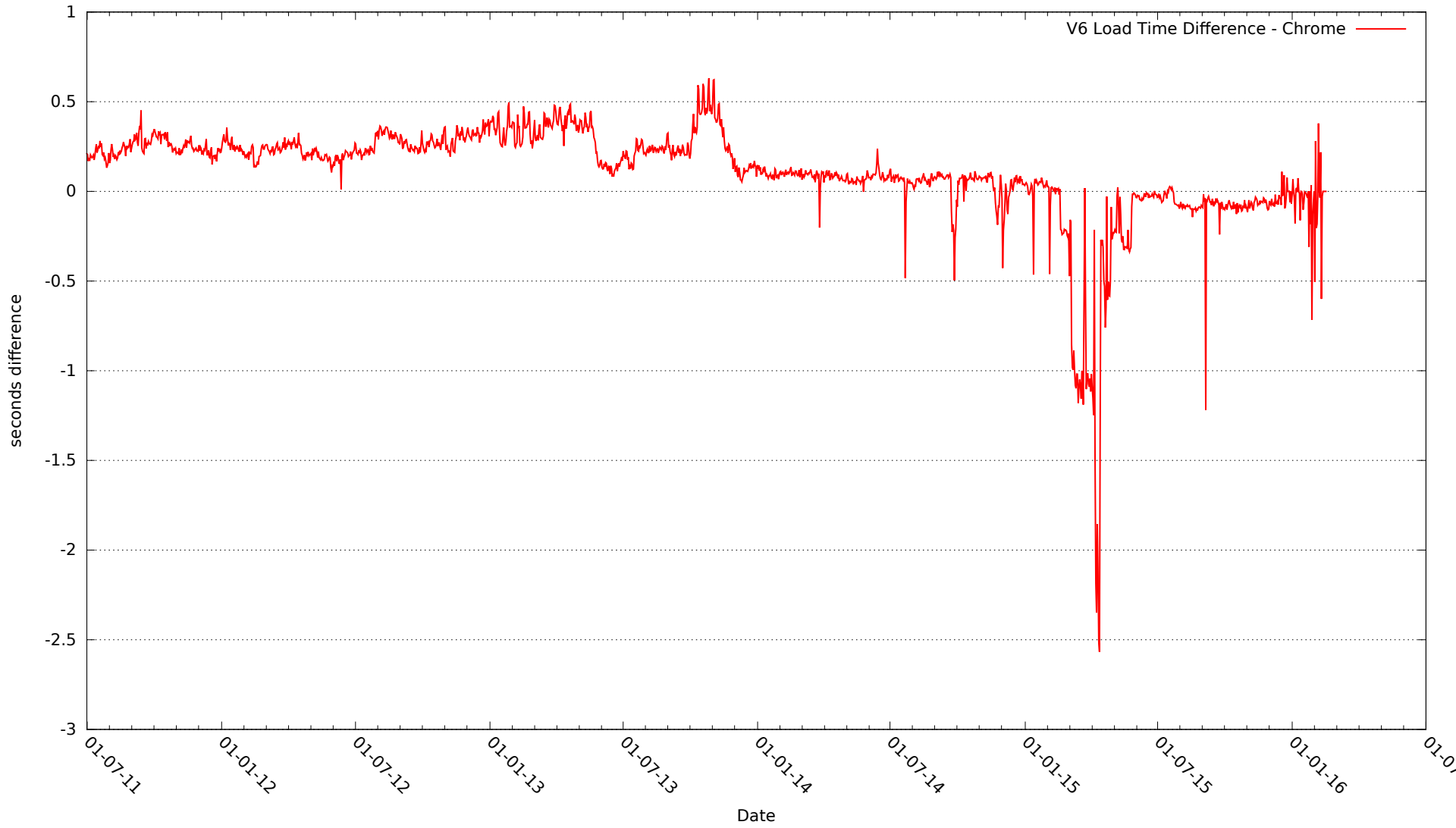
Avg V6 Load Time Differential (secs) - Chrome
