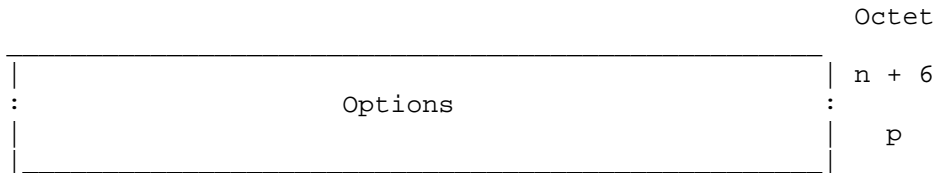
Figure 7: PDU Header -- Options Part
