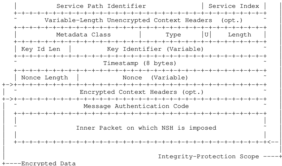
Figure 5: Scope of MAC#1
