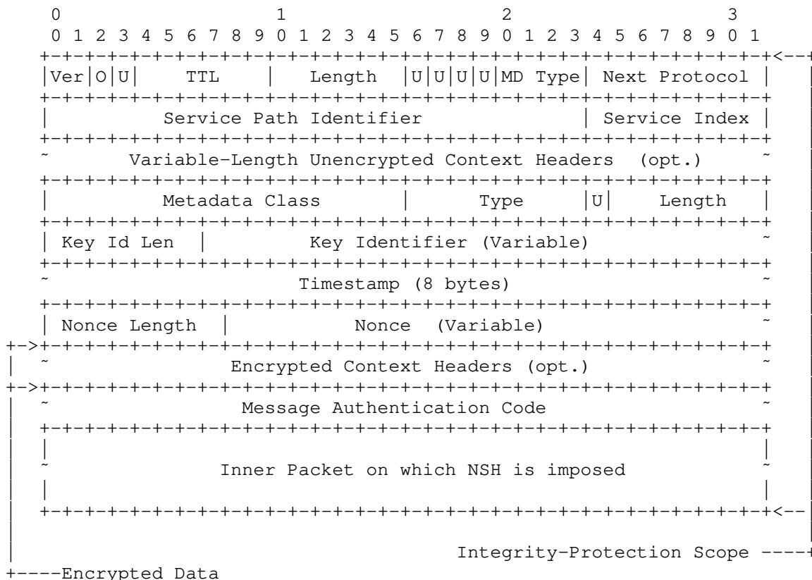
Figure 6: Scope of MAC#2
