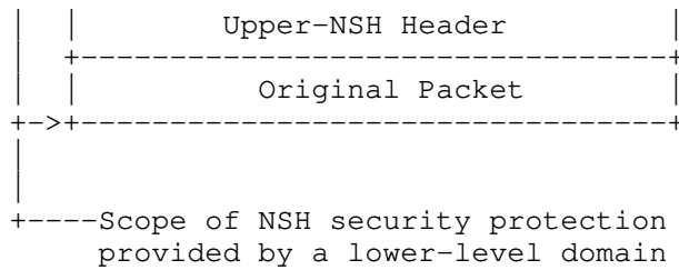
Figure 3: Encapsulation of NSH within NSH
