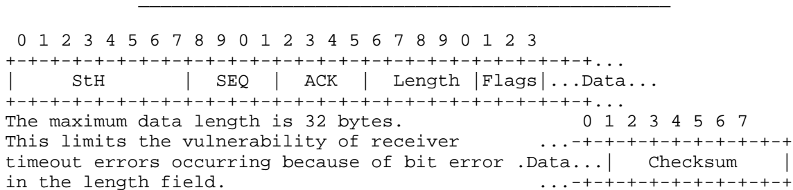
Figure D-1. SLIP Message Format
