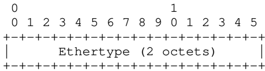
Figure 11: Protocol Type Sub-TLV Value Field
