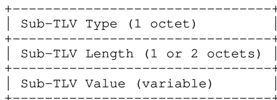
Figure 2: Encapsulation Sub-TLV
