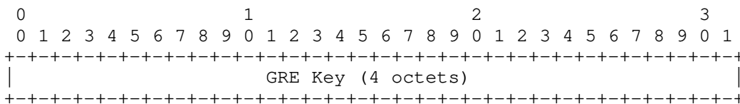
Figure 7: GRE Encapsulation Sub-TLV Value Field
