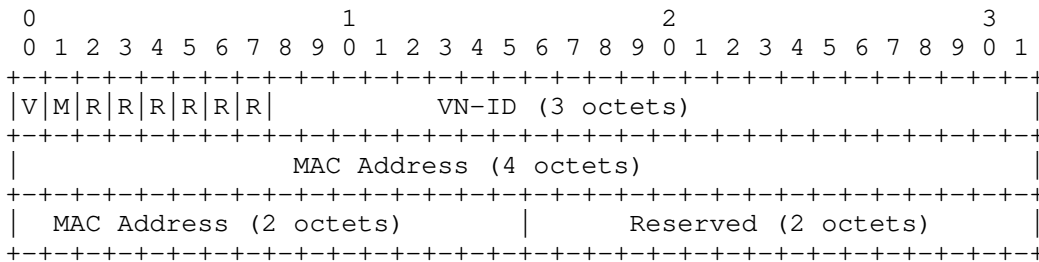
Figure 5: NVGRE Encapsulation Sub-TLV Value Field
