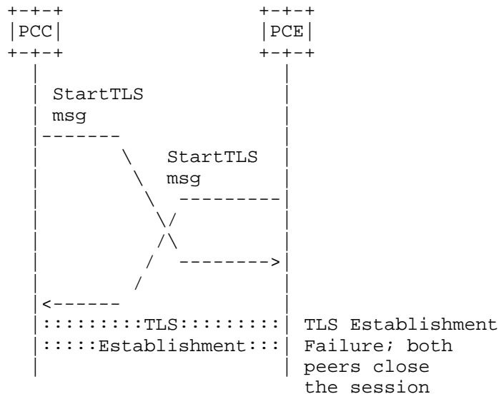
Figure 2: Both PCEP speakers support PCEPS (strict) but cannot establish TLS
