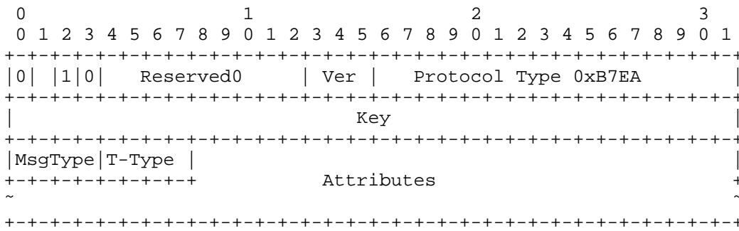
Figure 2: Format of Control Messages of GRE Tunnel Bonding
