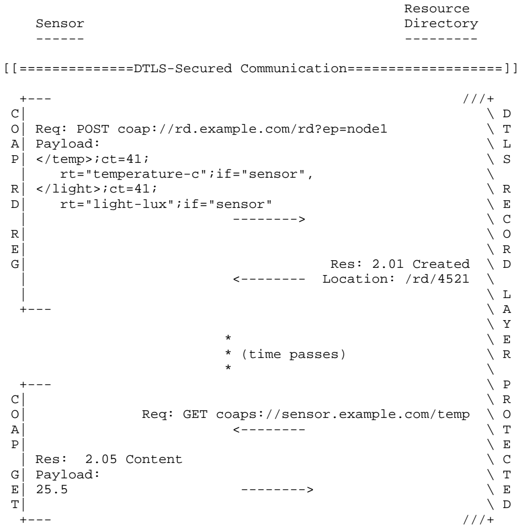
Figure 5: DTLS/CoAP Exchange Using Resource Directory: Part 2 -- CoAP/RD Exchange
