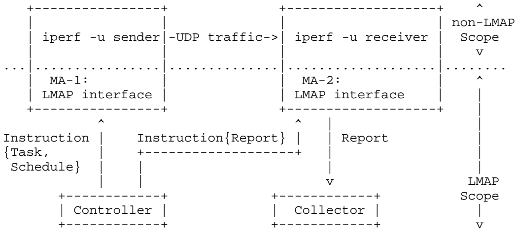
Figure 9: Schematic of LMAP-based Measurement System, with two Measurement Agents cooperating to measure UDP traffic
