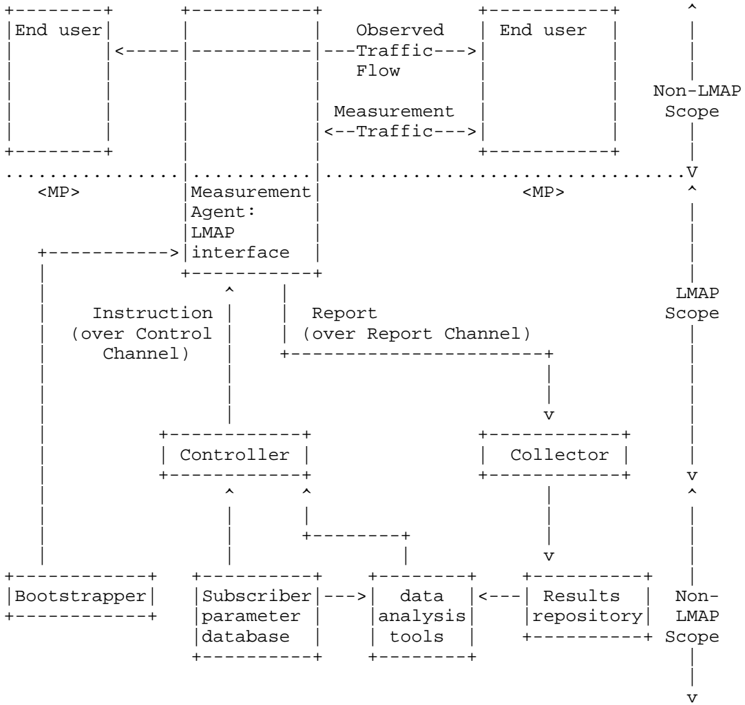
Figure 1: Schematic of main elements of an LMAP-based Measurement System (showing the elements in and out of the scope of initial LMAP work)
