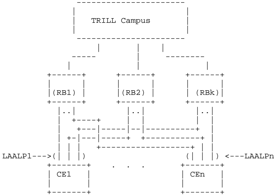
Figure 1: Active-Active Connection to TRILL Edge Rbridges
