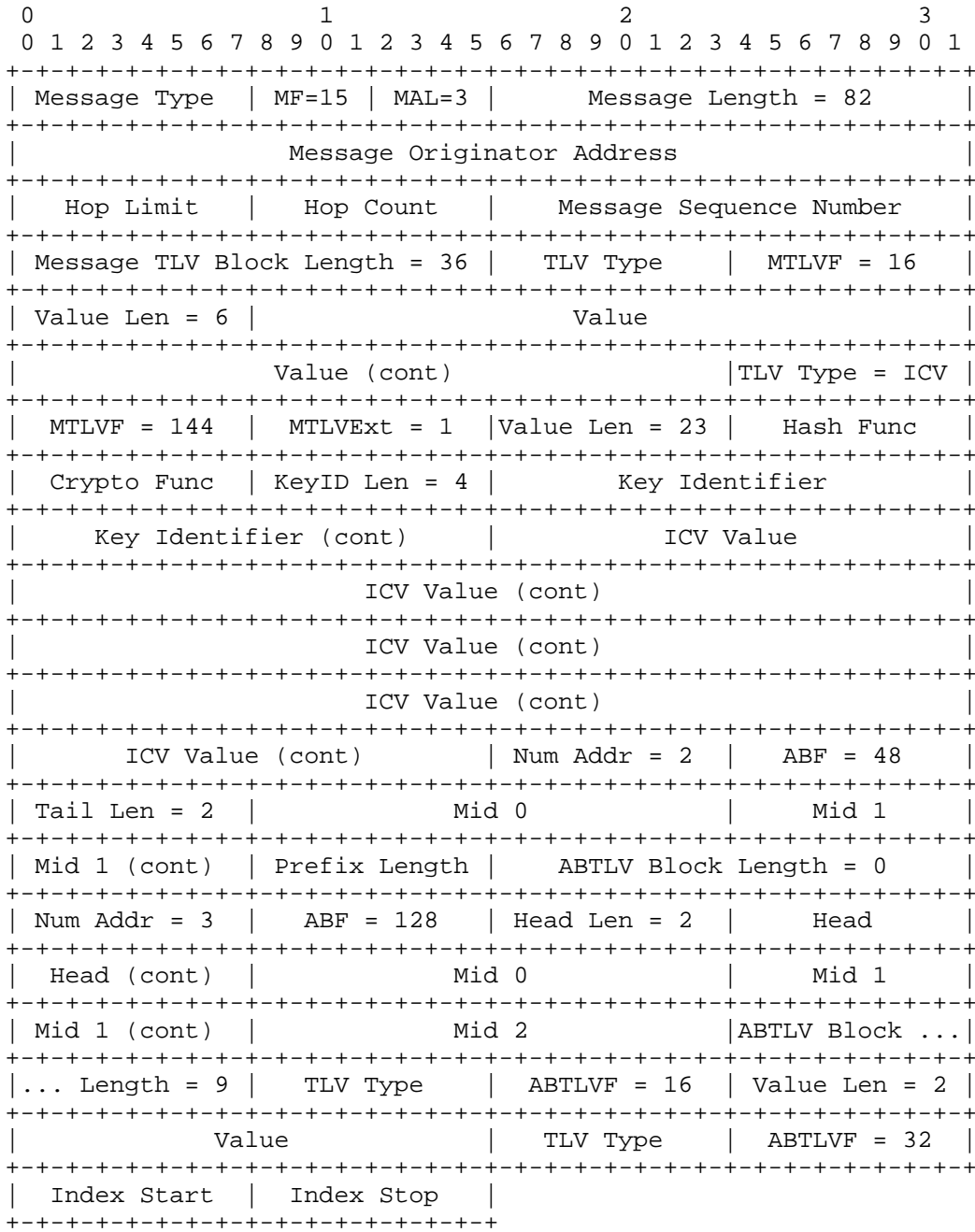
Figure 1: Example Message with ICV
