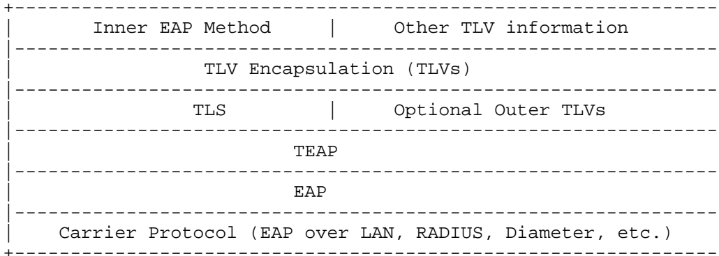
Protocol-Layering Model
