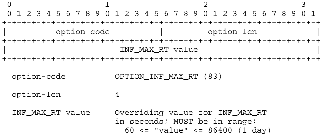
Figure 2: INF_MAX_RT Option Format
