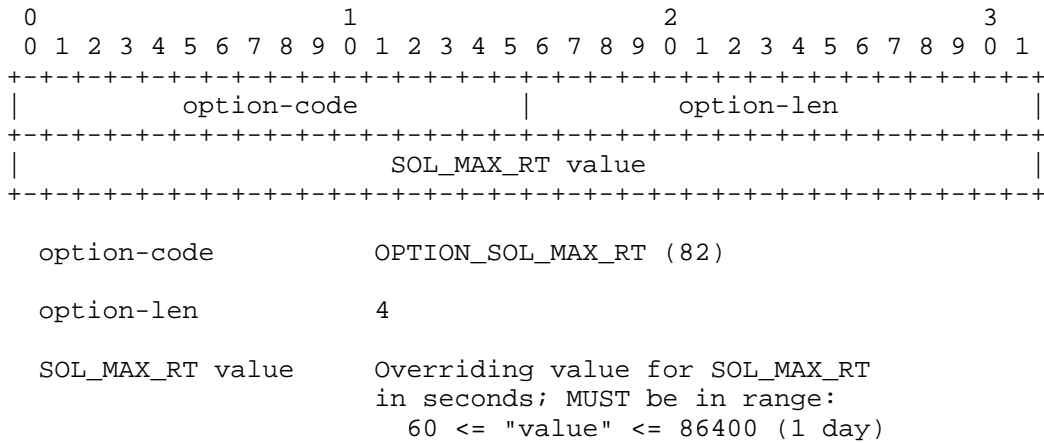
Figure 1: SOL_MAX_RT Option Format
