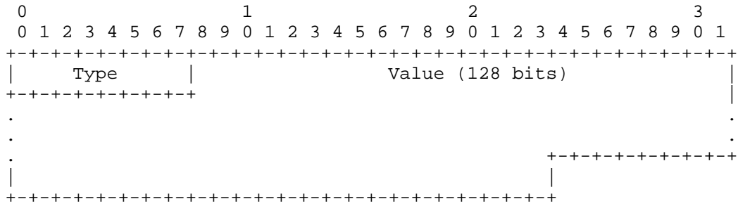
Figure 4: Format of the Authentication Information
