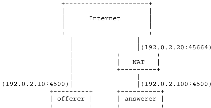
Figure 4: NAT-Traversal Scenario
